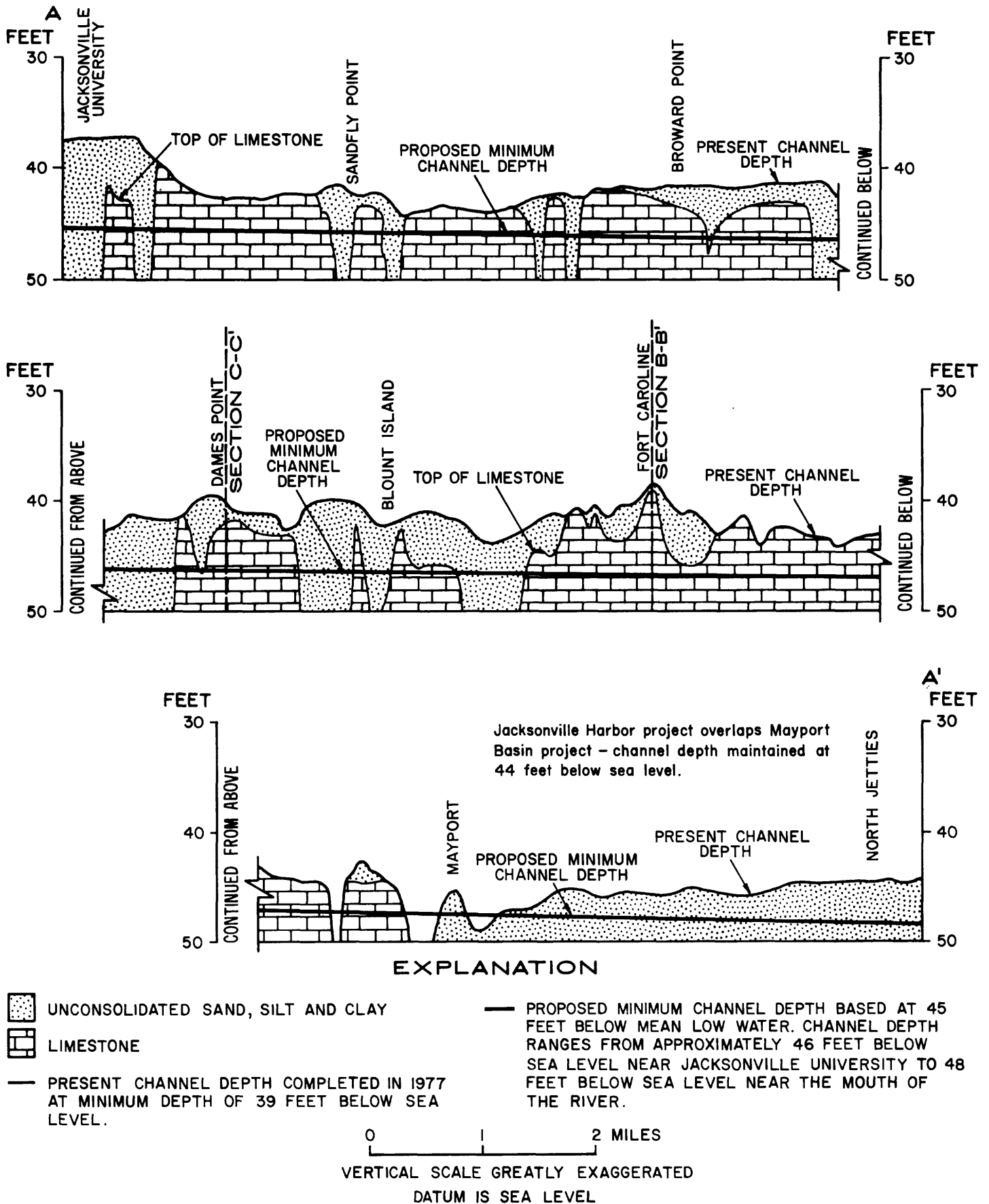
Figure 5.--Lithologic section A-A' along the St. Johns River.
