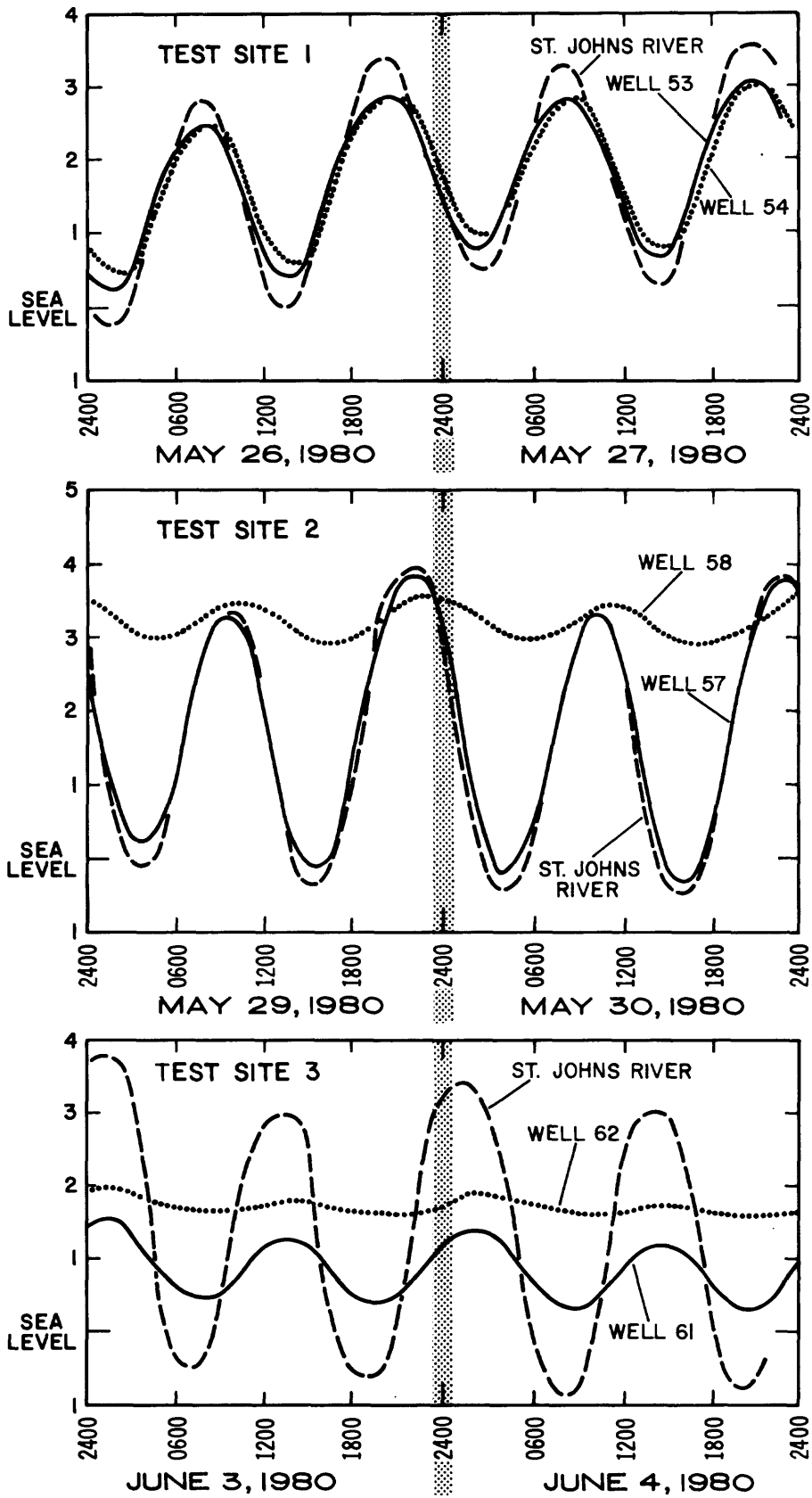
Figure 8.--Hydrographs of the St. Johns River and wells at test sites 1, 2, and 3.
