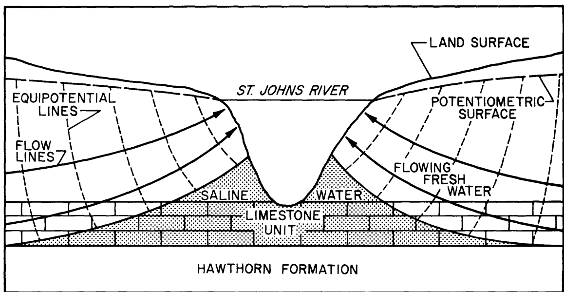
Figure 10.--Conceptual view of saline water-freshwater relations.
