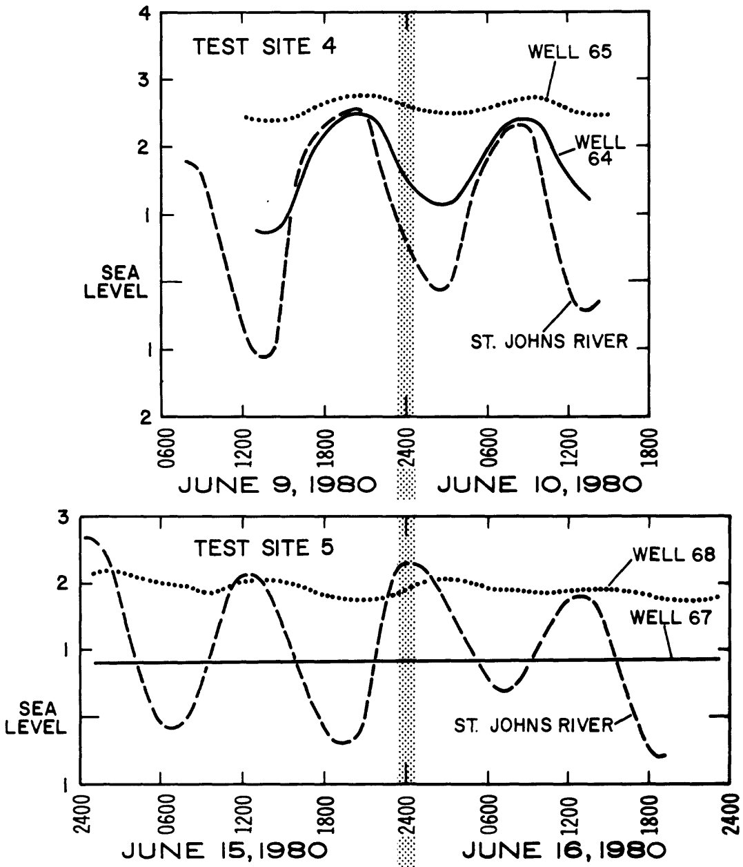
Figure 9.--Hydrographs of the St. Johns River and wells at test sites 4 and 5.
