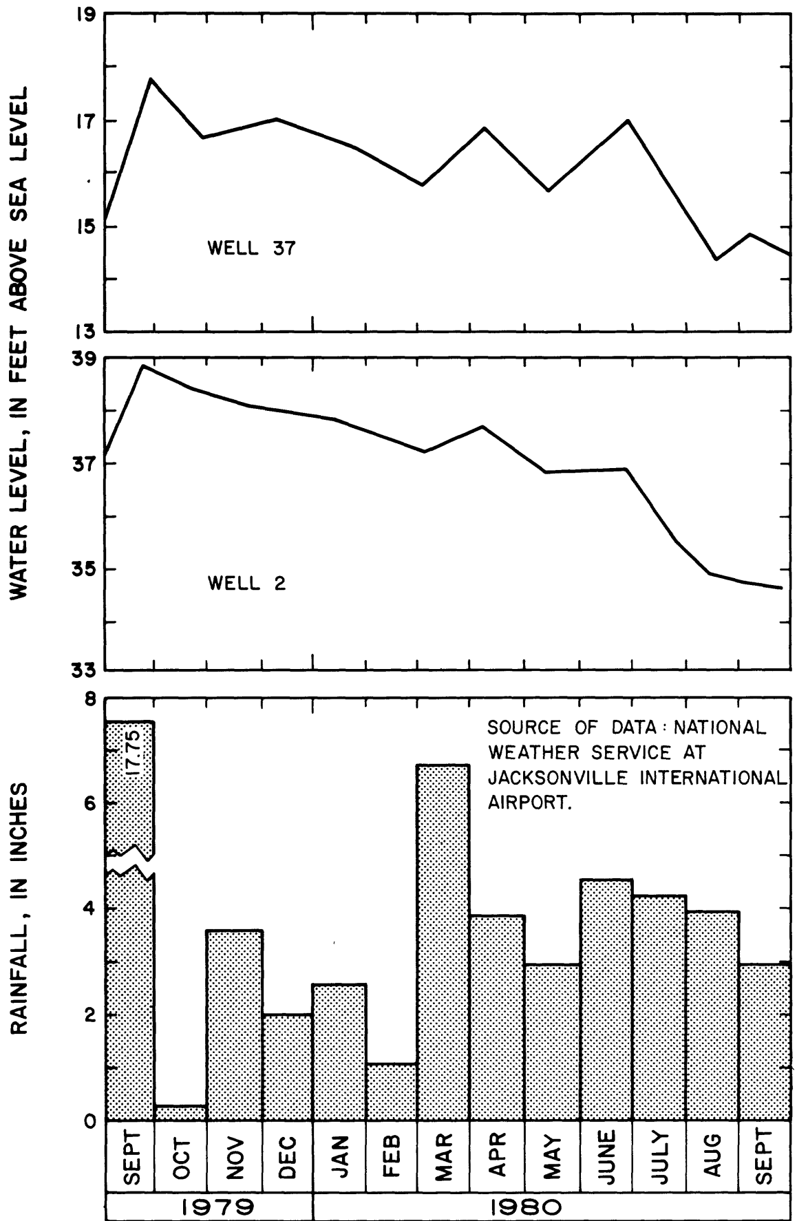
Figure 6.--Rainfall at Jacksonville and fluctuations of water levels in wells 37 and 2, 1979-80.
