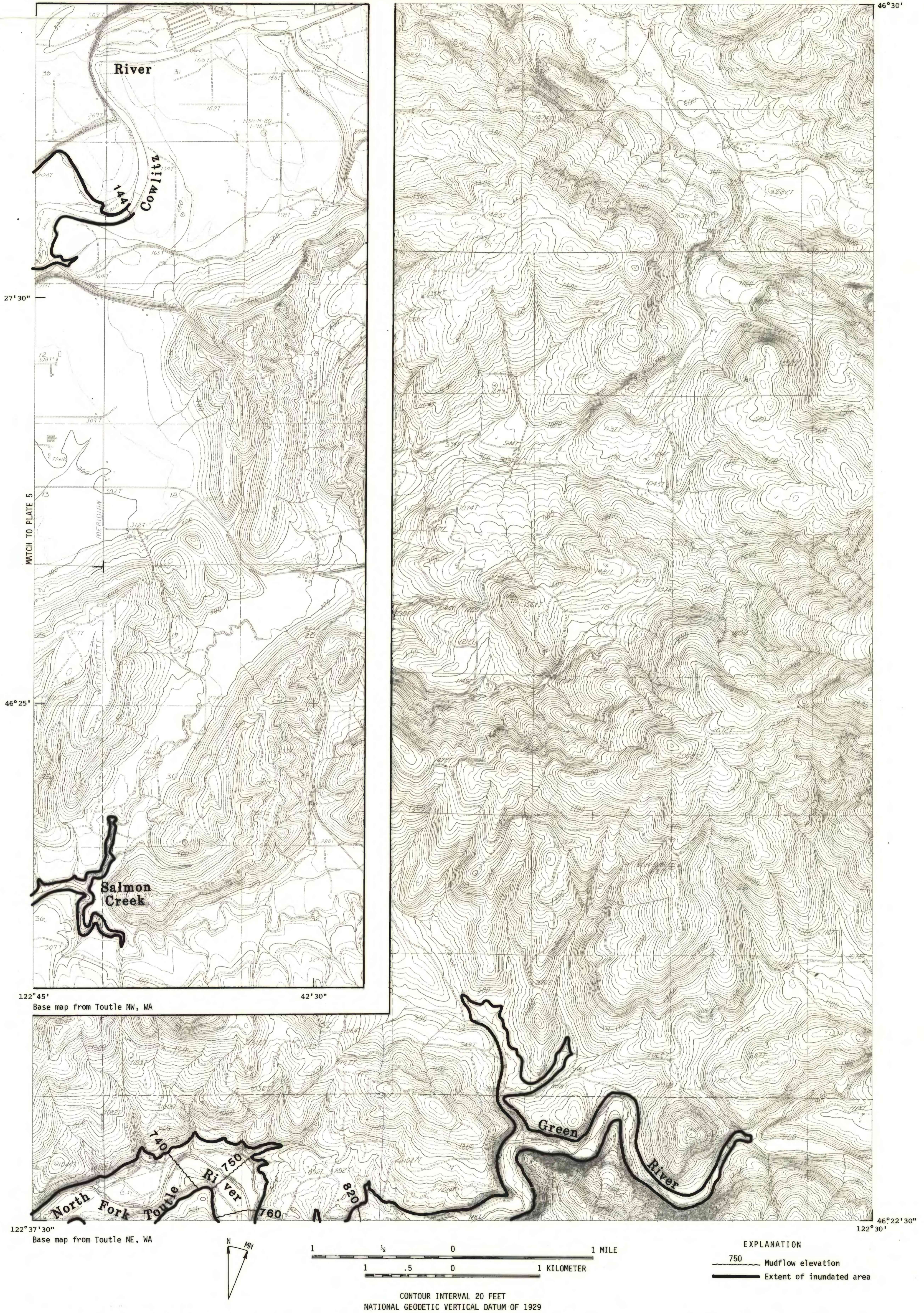
PLATE 4.-- Mudflow inundation map for N.F. Toutle River from river mile 6.1 to 10.5 in the vicinity of Kid Valley, and Cowlitz River from river mile 39.2 to 40.1 in vicinity of Toledo.
