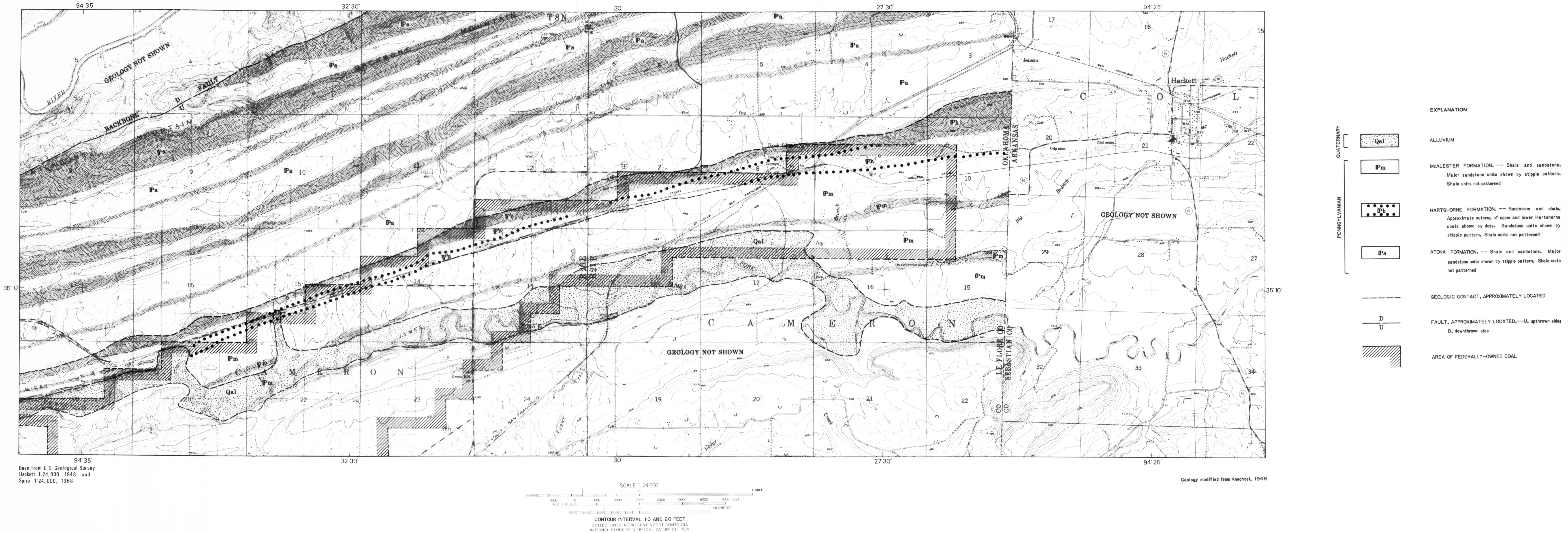
GEOLOGIC MAP OF THE ROCK ISLAND AREA, LE FLORE COUNTY, OKLAHOMA
