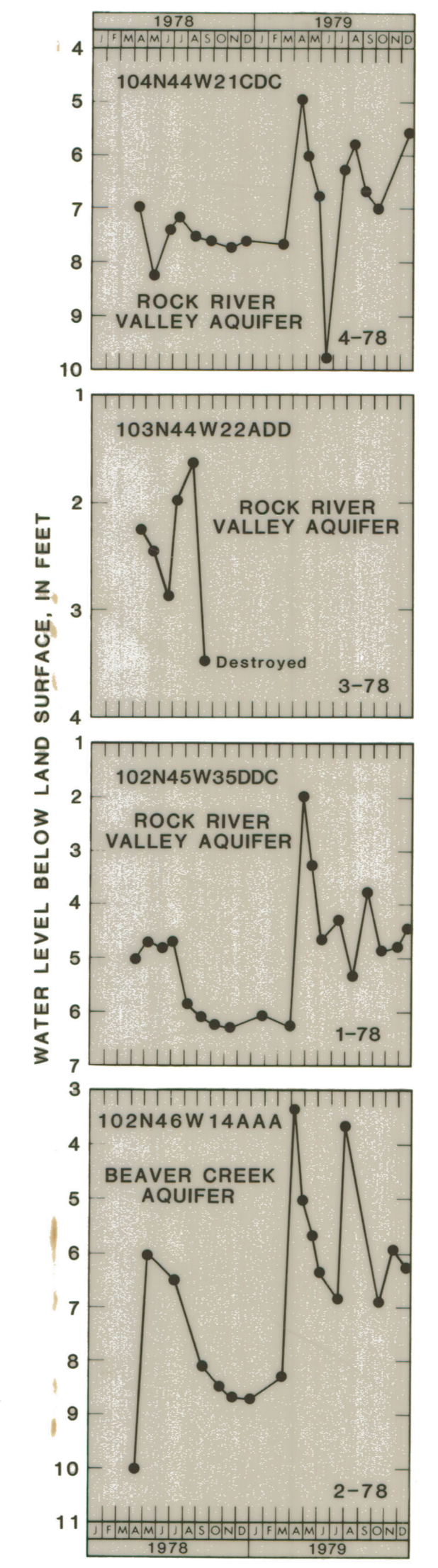
WATER LEVEL FLUCTUATIONS IN FOUR WELLS
