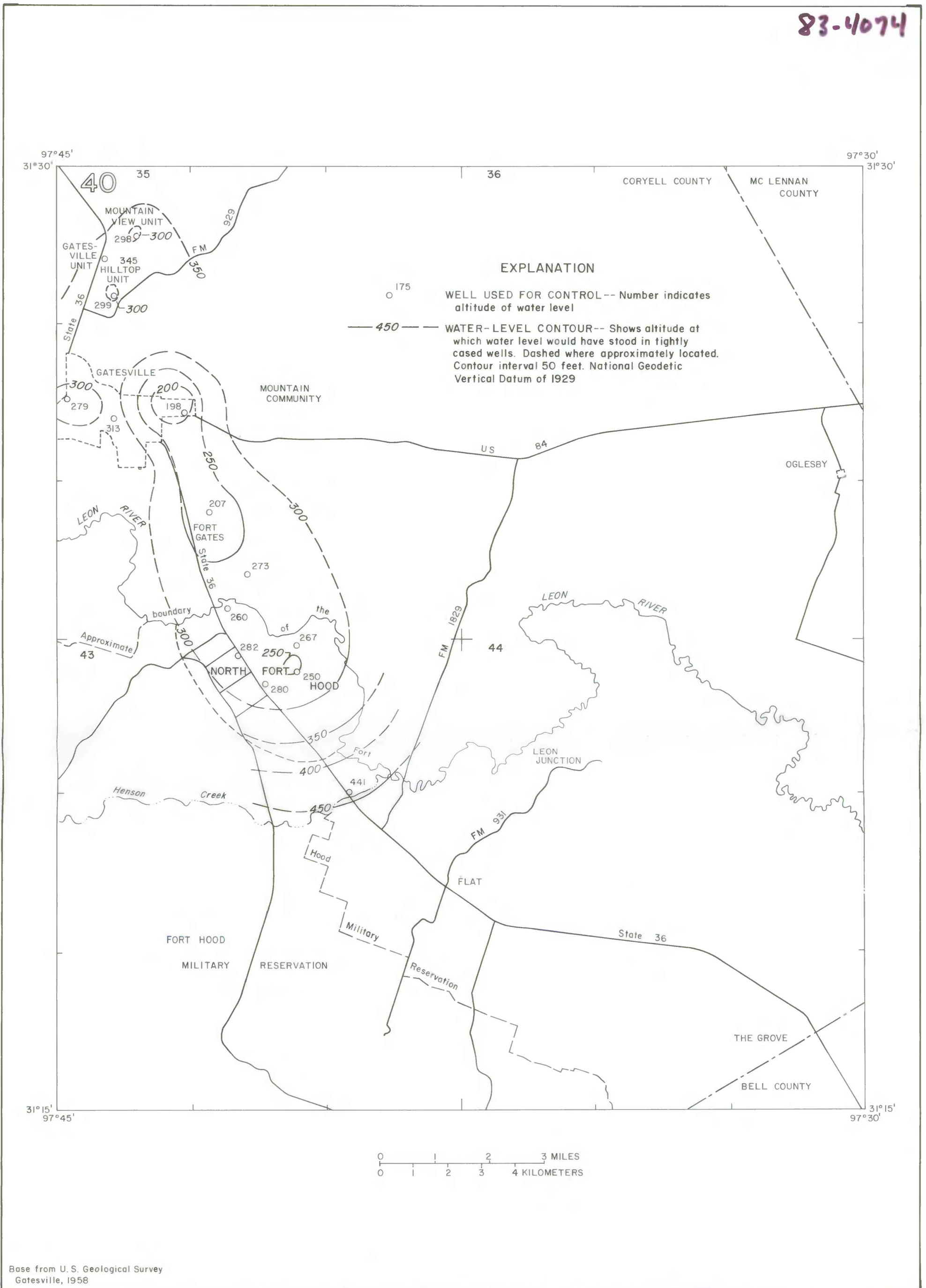
Figure 5.—Altitude of approximate water levels in wells screened in the Hensell and Hosston Members of the Travis Peak Formation (of Klemt, Perkins, and Alvarez, 1975), September–November, 1982.
