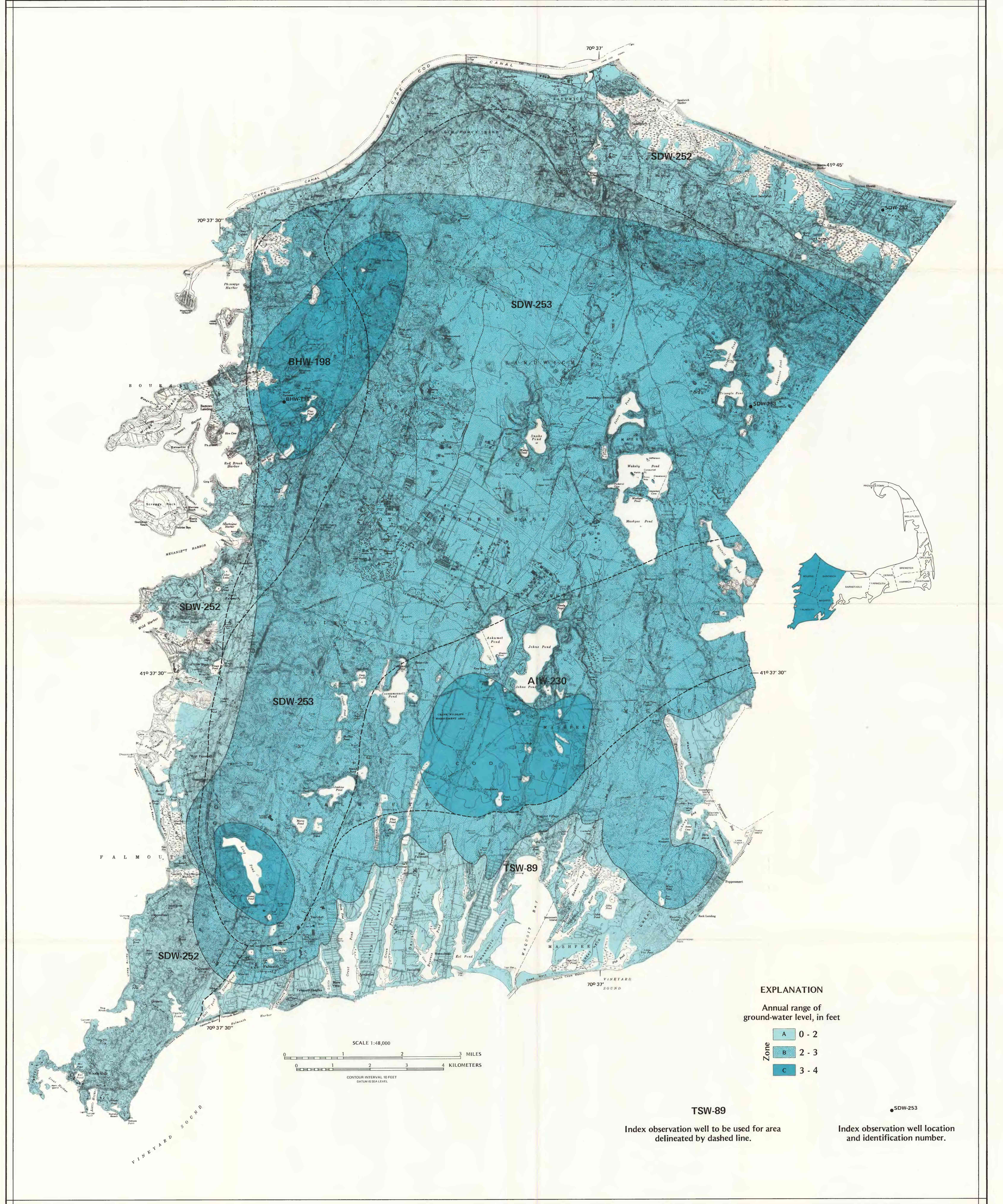
PLATE 1. ANNUAL RANGES OF GROUND-WATER LEVEL AND INDEX-WELL AREAS FOR CAPE COD, MASSACHUSETTS: TOWNS OF BOURNE, FALMOUTH, MASHPEE, AND SANDWICH.
