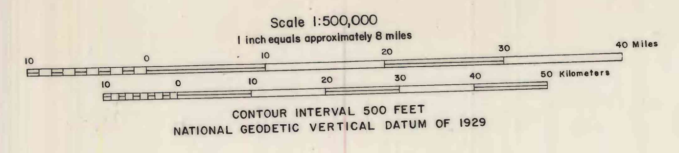
MAP SHOWING OUTCROPS OF PRE-QUATERNARY BASALTIC ROCKS, BASIN AND RANGE PROVINCE, ARIZONA Compiled by William D. Johnson, Jr. and Robert B. Scarborough 1984
