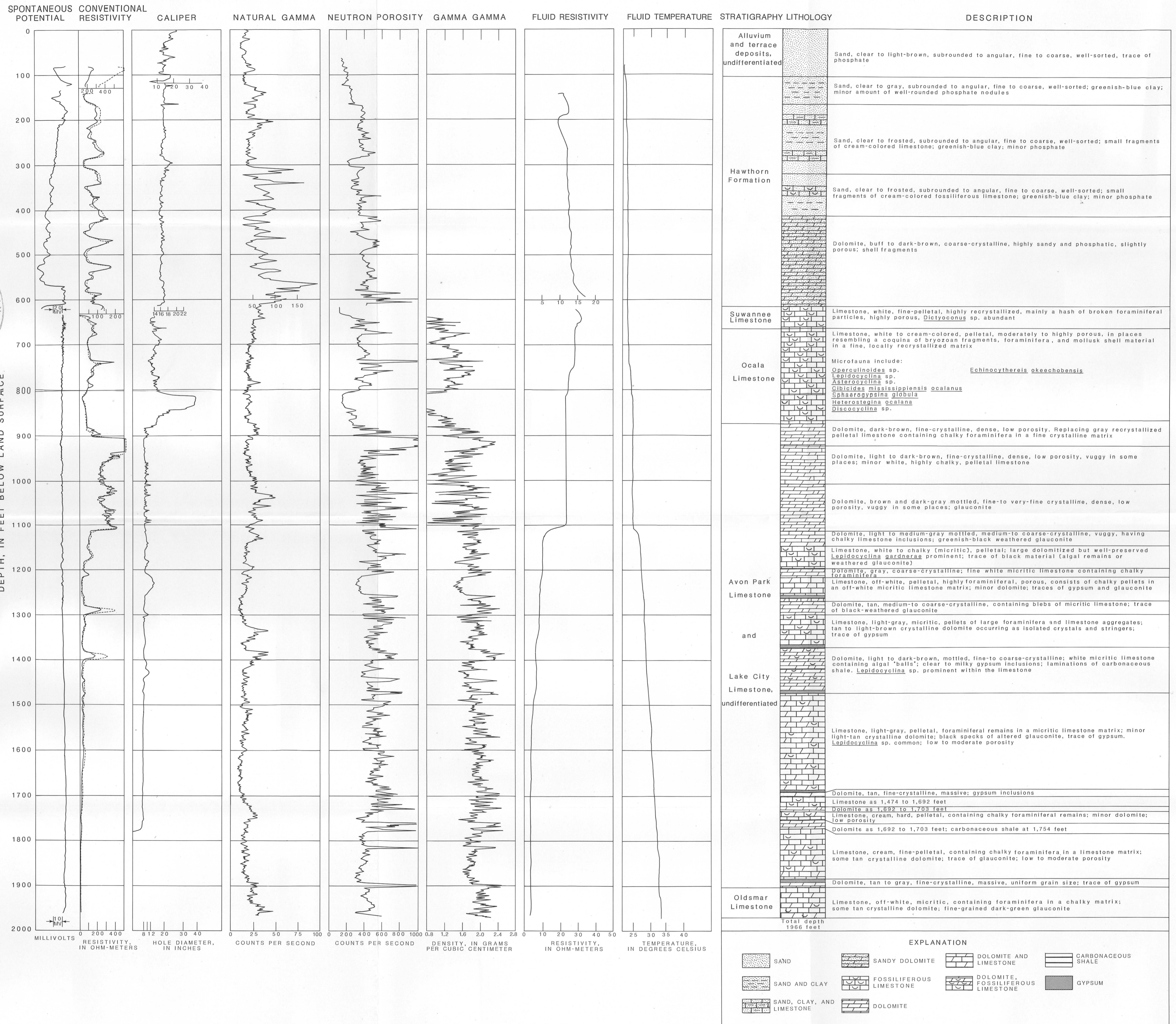
GEOPHYSICAL LOGS, STRATIGRAPHIC SECTION, AND LITHOLOGIC DESCRIPTION OF TEST WELL 2, WARE COUNTY, GEORGIA.
