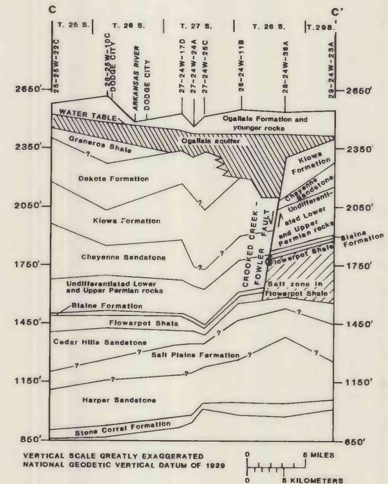
Figure 6.--North-south geologic section showing stratigraphic relationship of the Ogallala aquifer to underlying rocks. Trace of section is shown in figure 7.
