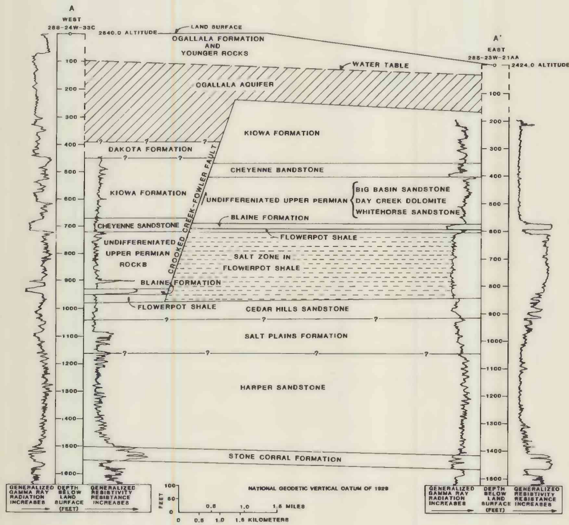
Figure 4.--Geophysical logs and geohydrologic correlations of stratigraphy in study area. Trace of section shown on figure 3.
