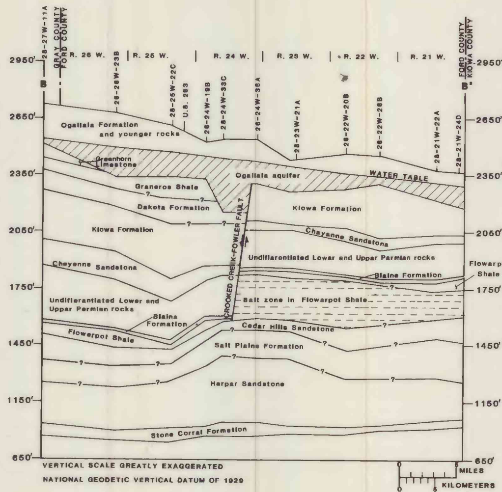
Figure 5.--East-west geologic section showing stratigraphic relationship of the Ogallala aquifer to underlying rocks. Trace of section is shown in figure 7.
