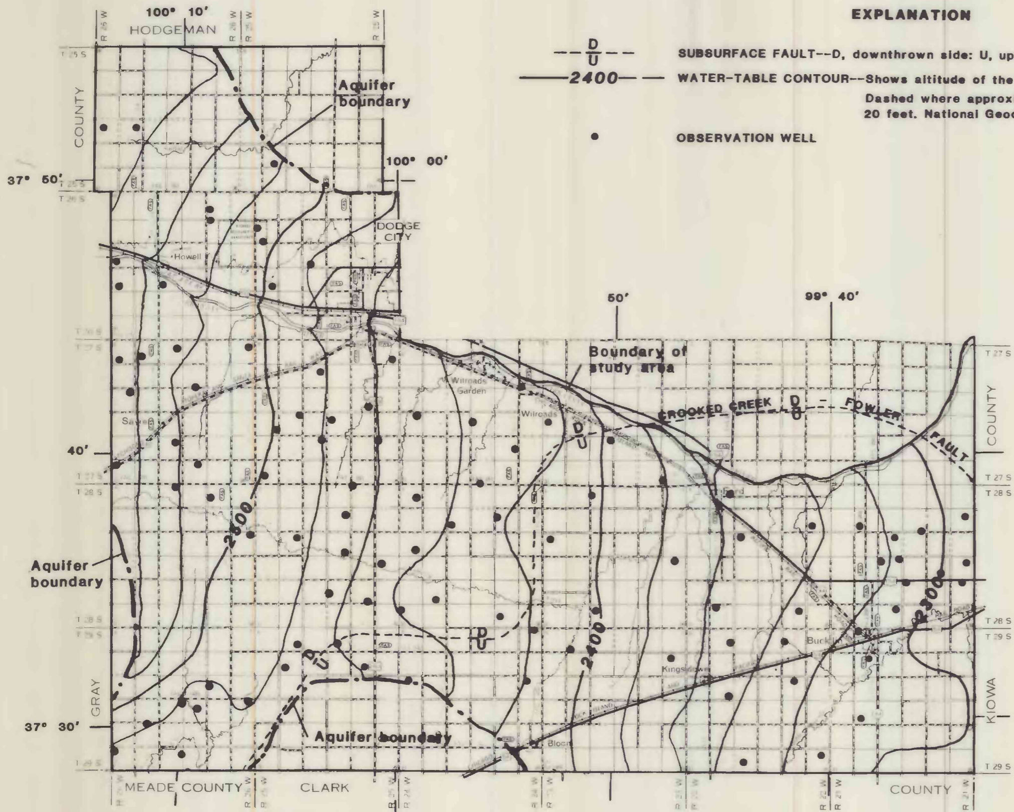
Figure 9.--Configuration of water table in the Ogallala aquifer, January 1981.
