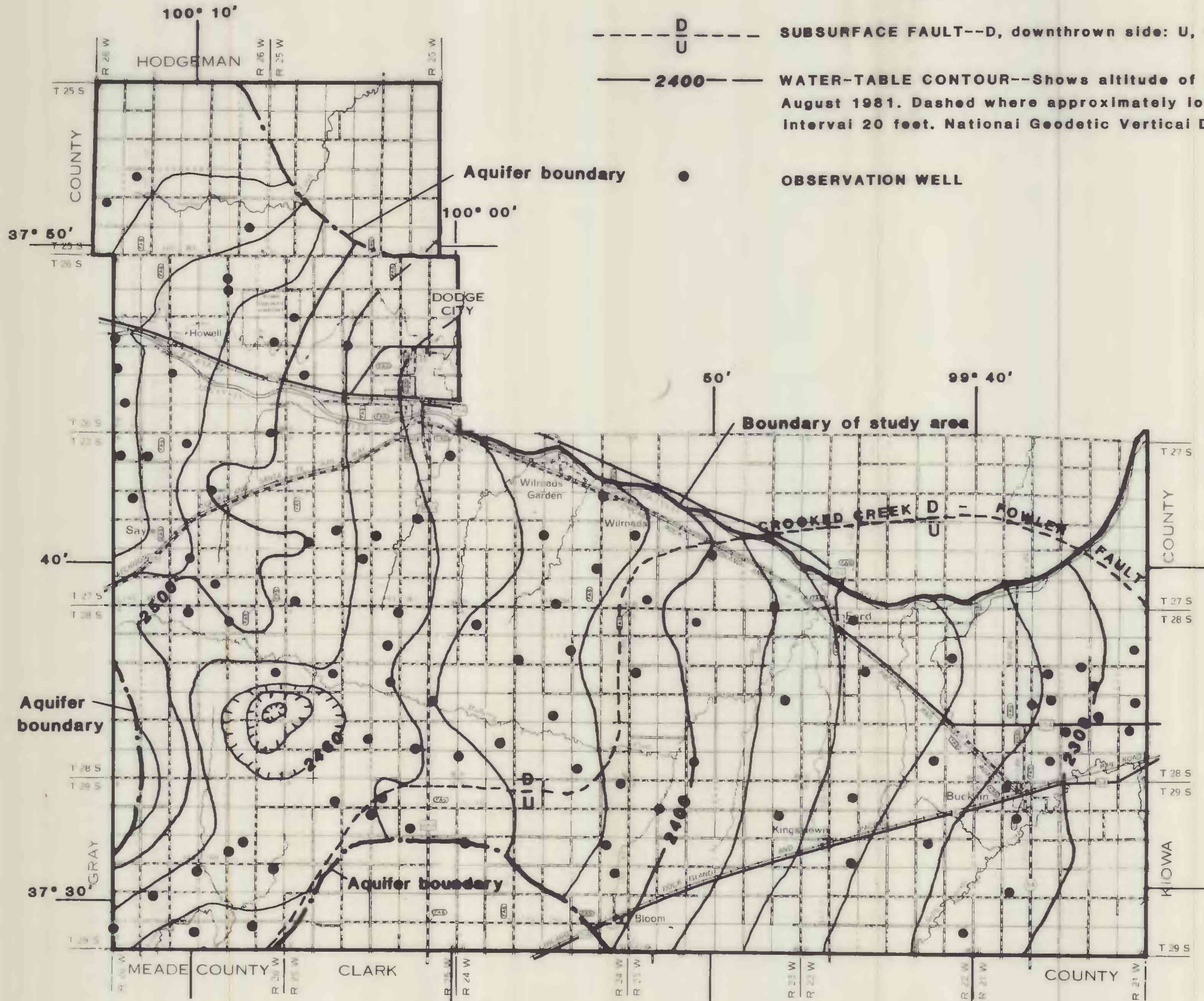
Figure 10.--Configuration of water table in the Ogallala aquifer, August 1981.
