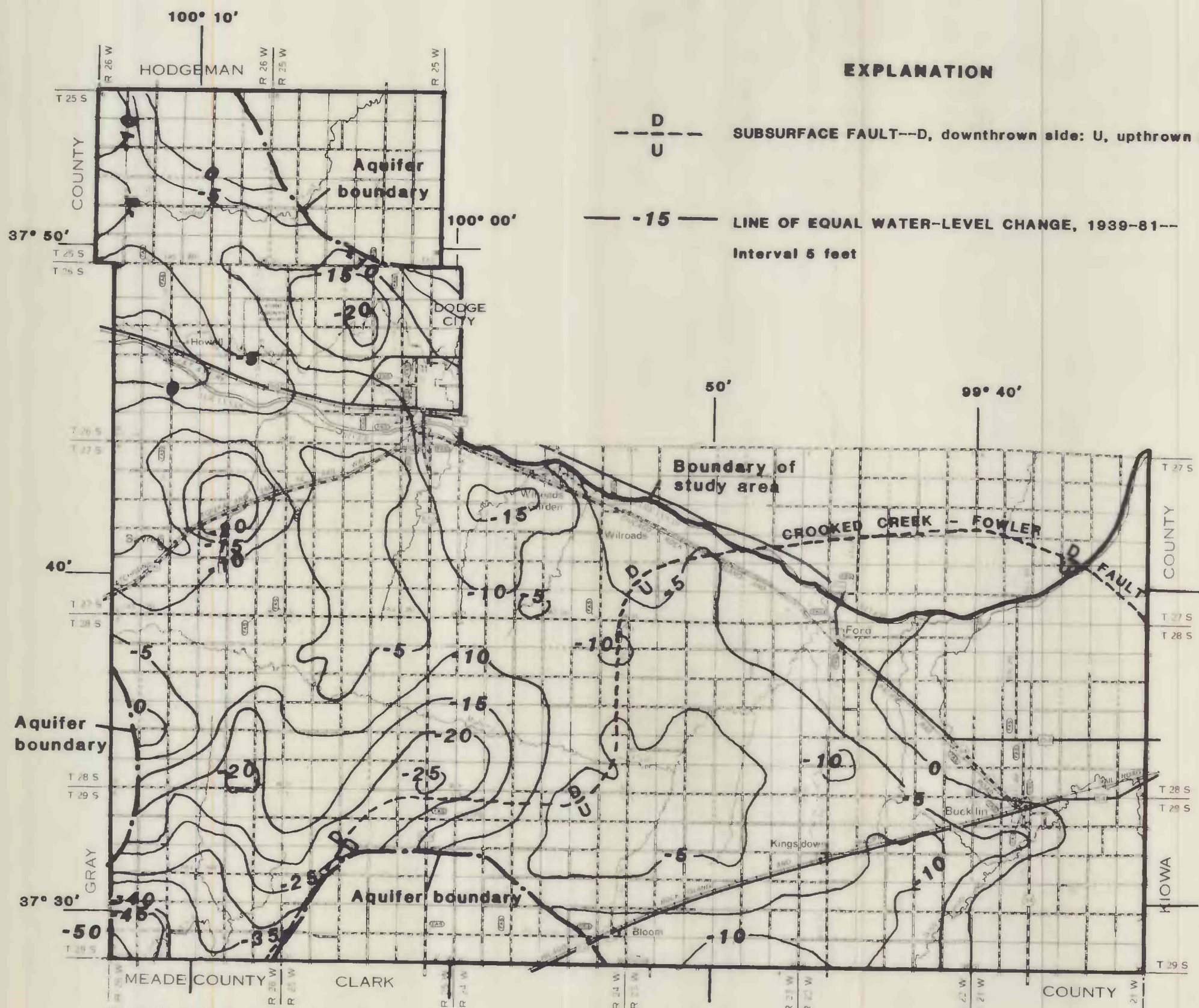
Figure 13.--Water-level changes in the Ogallala aquifer, 1939-81.
