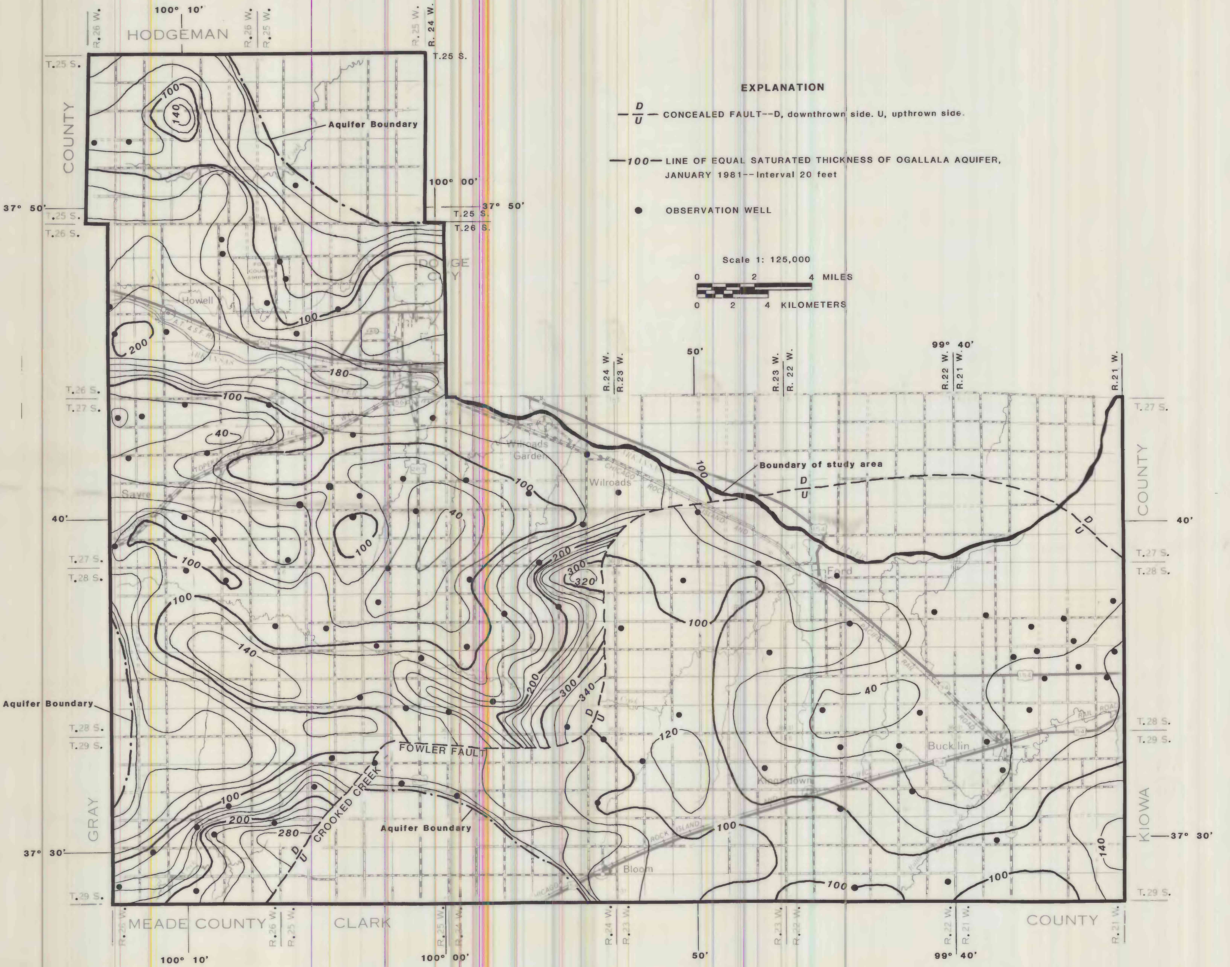
MAP SHOWING SATURATED THICKNESS OF THE OGALLALA AQUIFER IN FORD COUNTY, SOUTHWESTERN KANSAS
