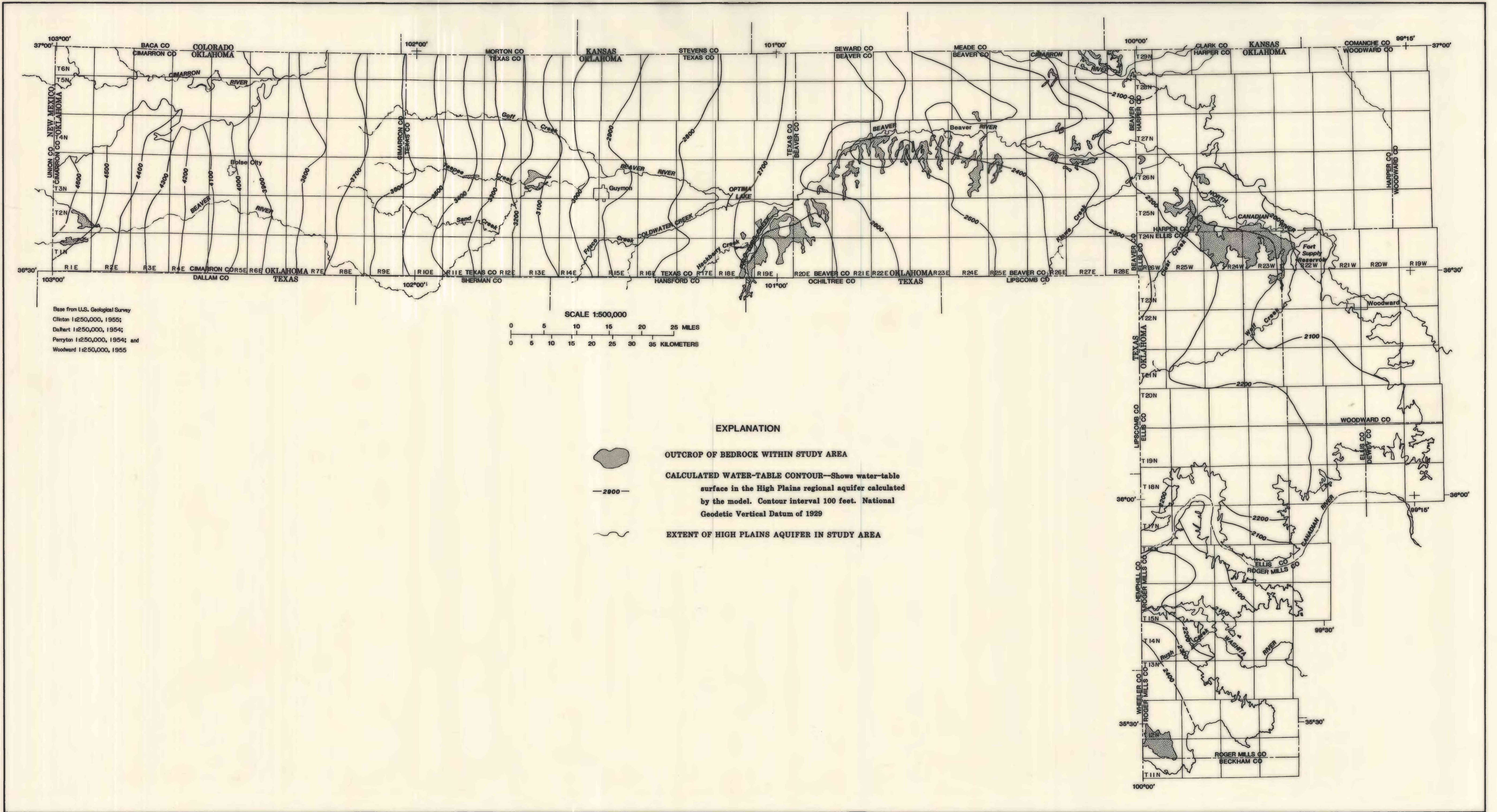
Plate 5.--Map showing calculated 1993 water levels in the High Plains regional aquifer, northwestern Oklahoma.
