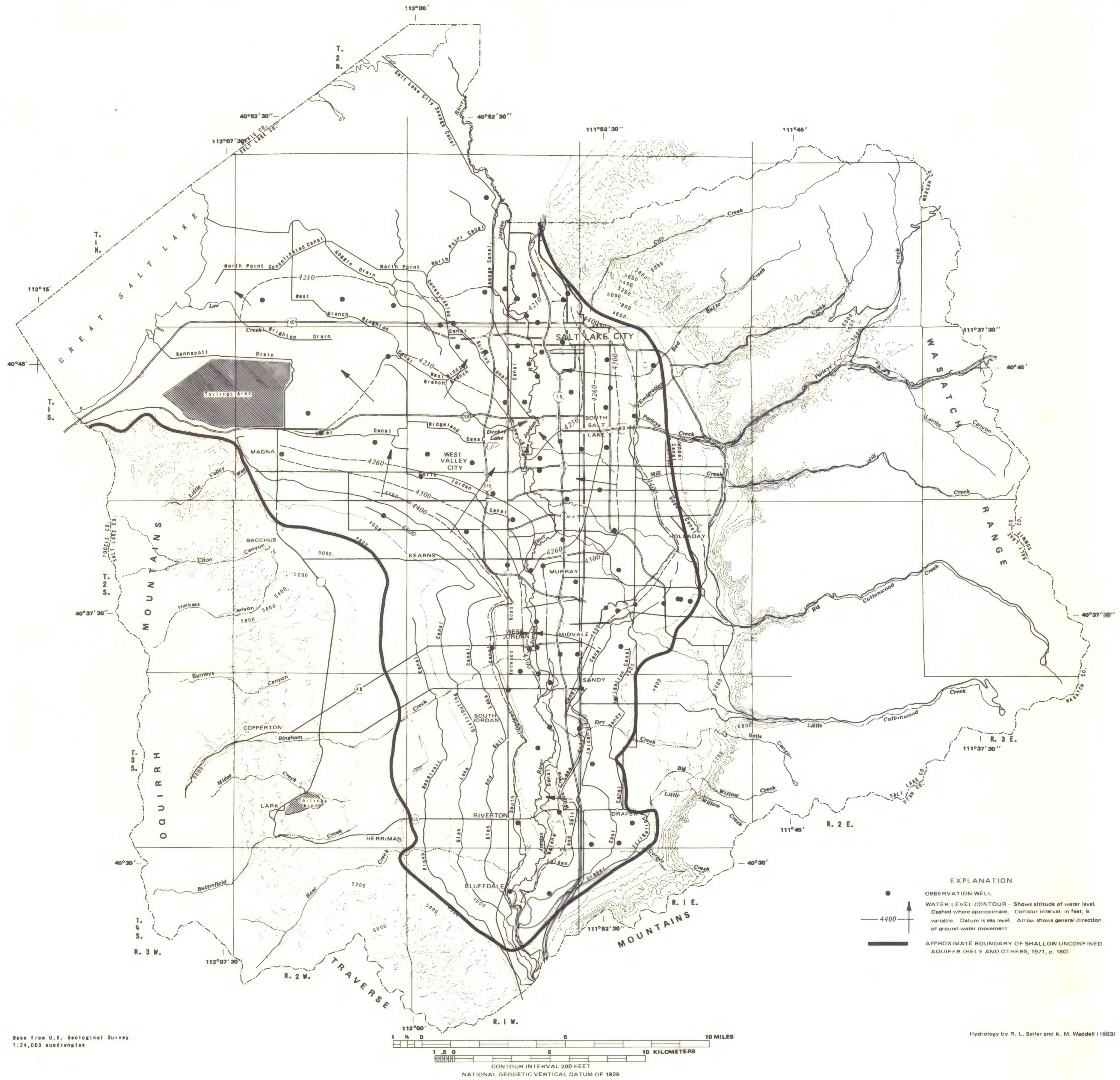
MAP SHOWING WATER-LEVEL CONTOURS FOR THE SHALLOW-UNCONFINED AQUIFER AND DIRECTION OF FLOW IN DECEMBER 1982 IN SALT LAKE VALLEY, UTAH.
