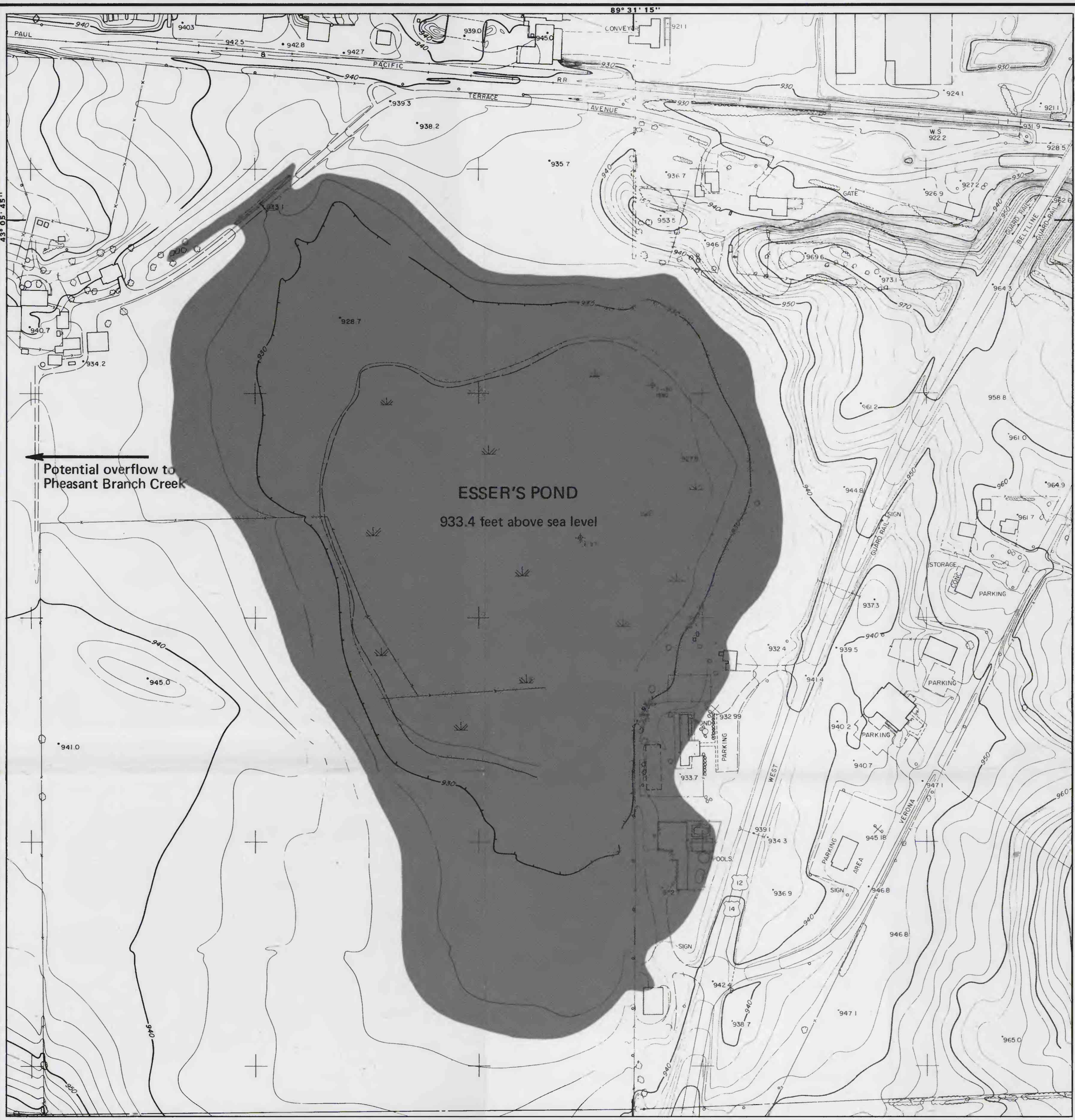
Peak daily mean stage at Tiedeman's, Stricker's, and Esser's Ponds, Middleton, Wisconsin, for the 100-year recurrence interval rainfall record (April 15 - November 5).
