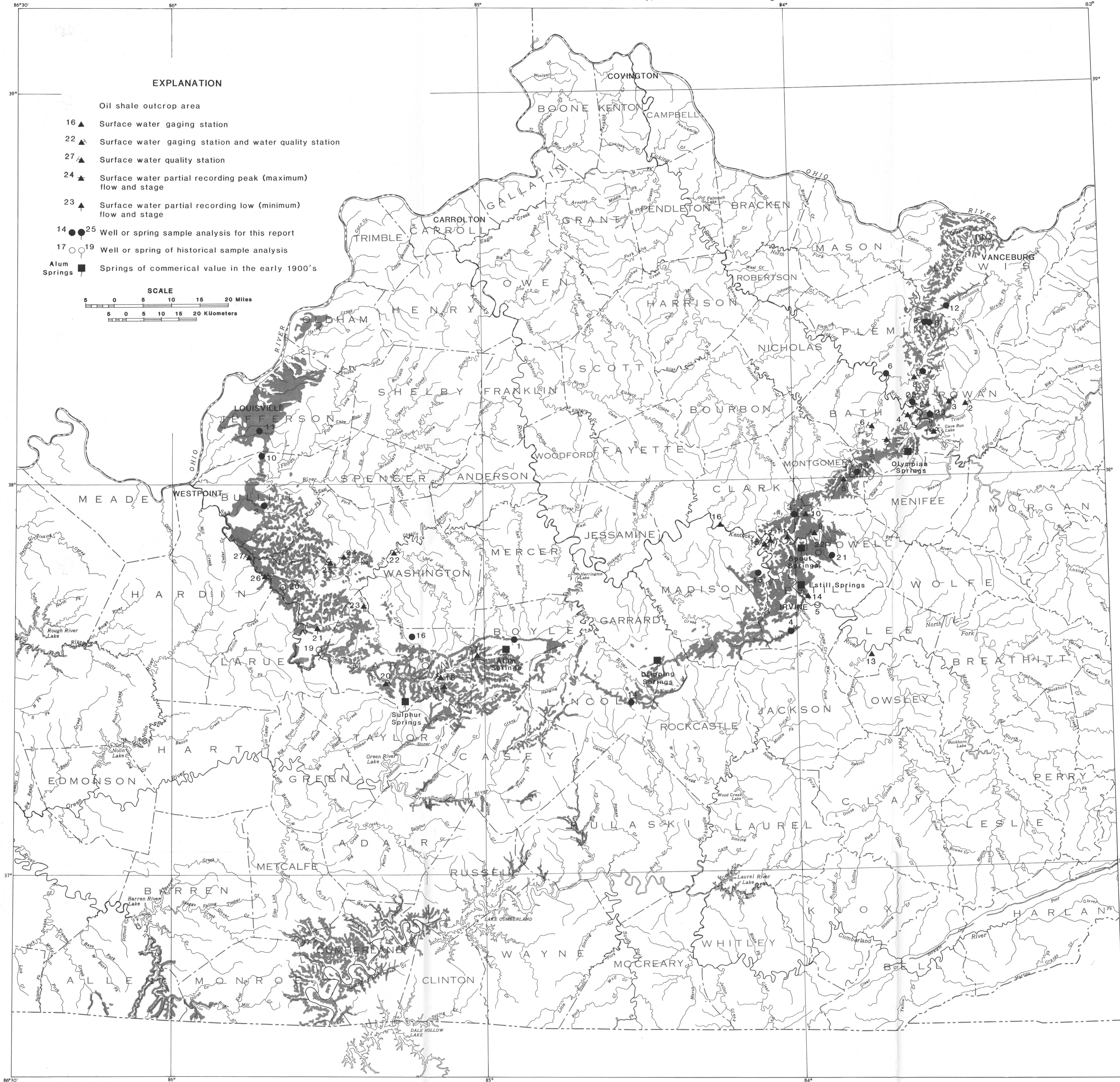
LOCATION OF OIL SHALE OUTCROP AREAS AND GROUND AND SURFACE WATER SITES, CENTRAL KENTUCKY.
