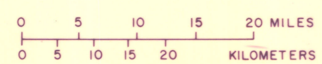
PLATE 2.--MAP SHOWING SELECTED WELLS, WATER LEVELS IN, AND THICKNESS OF THE CAPITAN AQUIFER, TEXAS AND NEW MEXICO.
