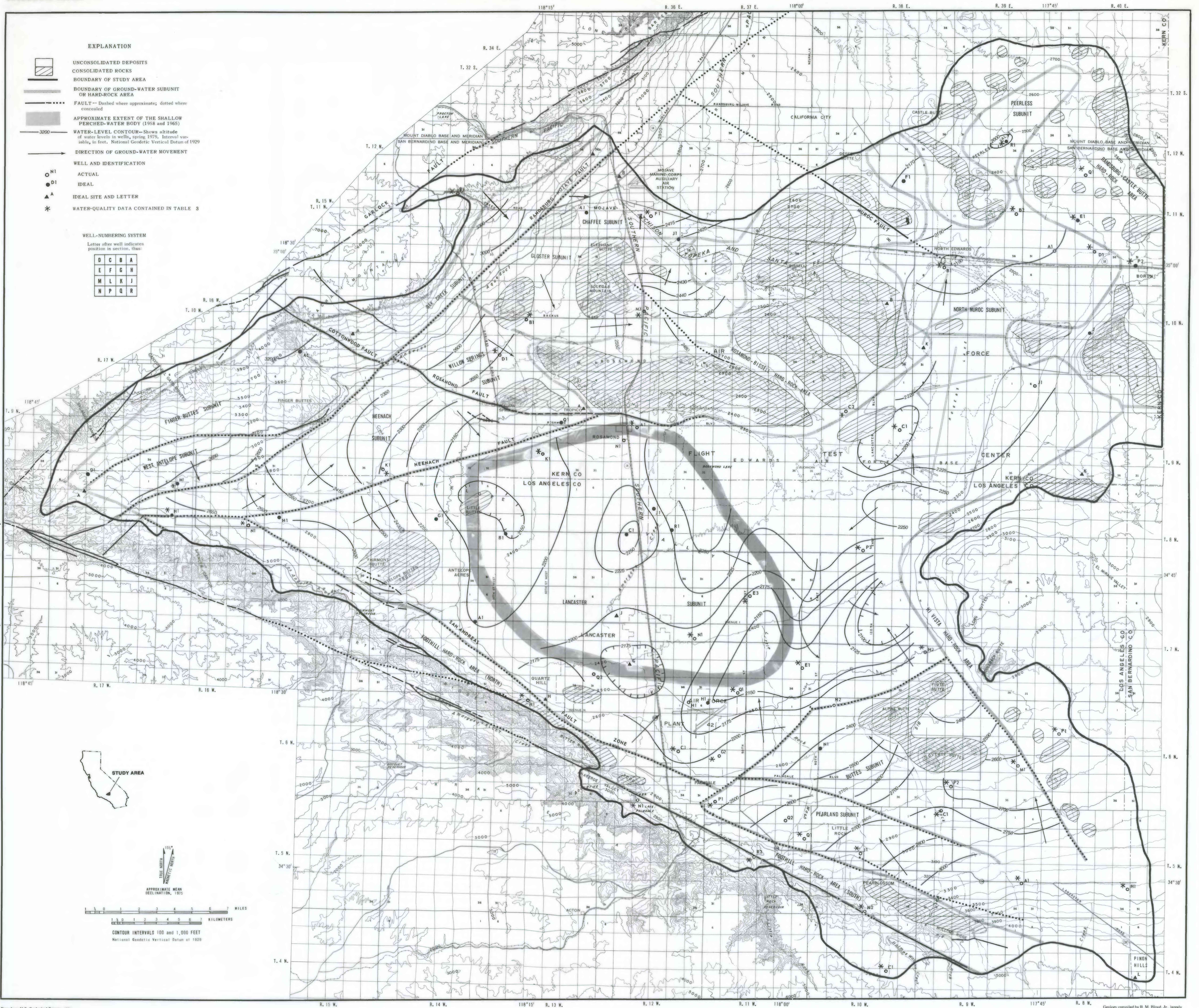
MAP SHOWING LOCATION OF PROPOSED NETWORK AND GROUND-WATER SUBDIVISIONS IN ANTELOPE VALLEY, CALIFORNIA
