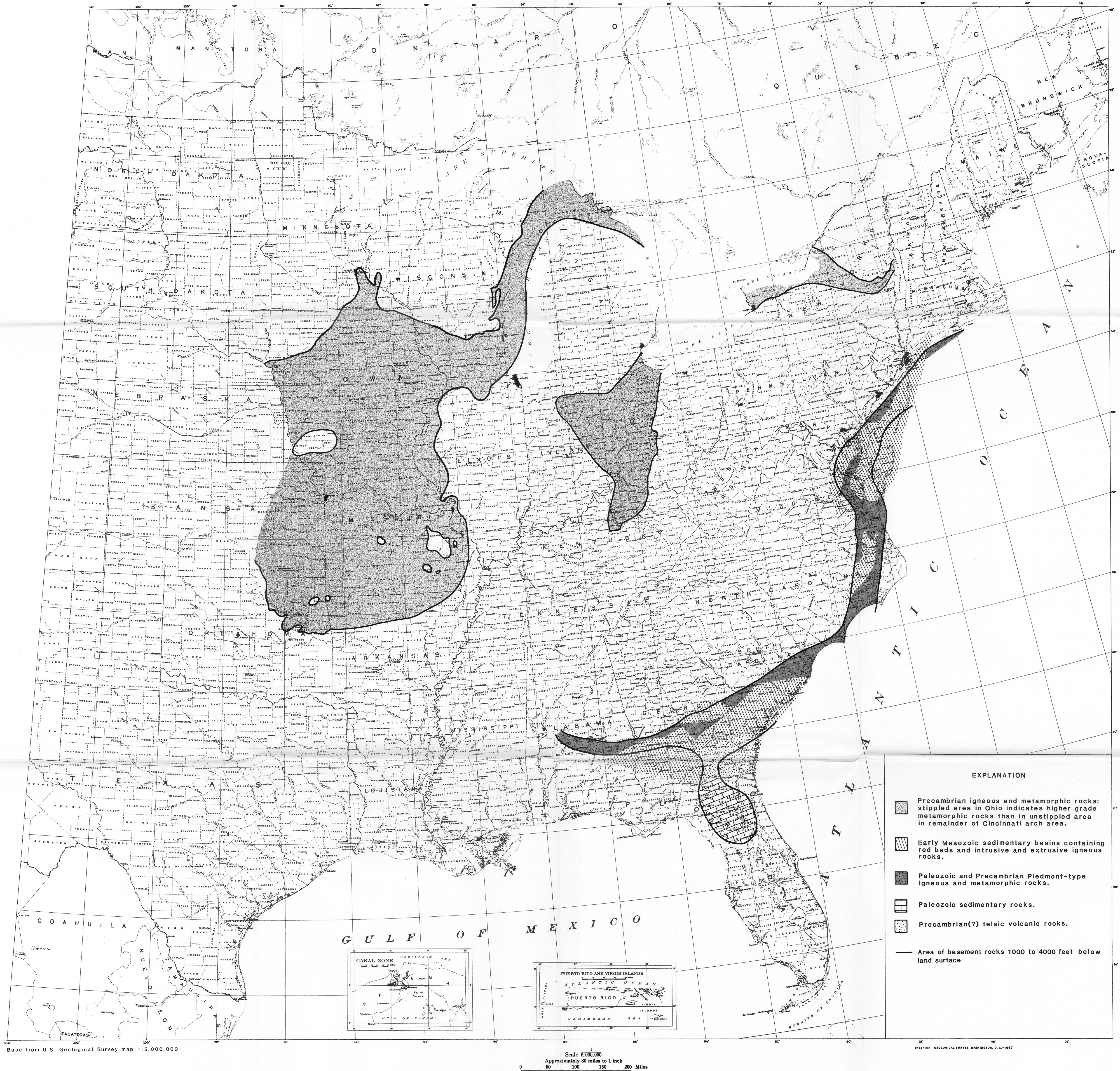
LITHOLOGIC CHARACTERISTICS OF BASEMENT ROCKS IN SELECTED AREAS OF THE EASTERN UNITED STATES. LITHOLOGIC TYPES IN THE ATLANTIC COASTAL PLAIN MODIFIED FROM CHOWN AND WILLIAMS (1983, PL. 1) AND WENTWORTH AND MERGNER-KEEFER (1983, PL. 1).
