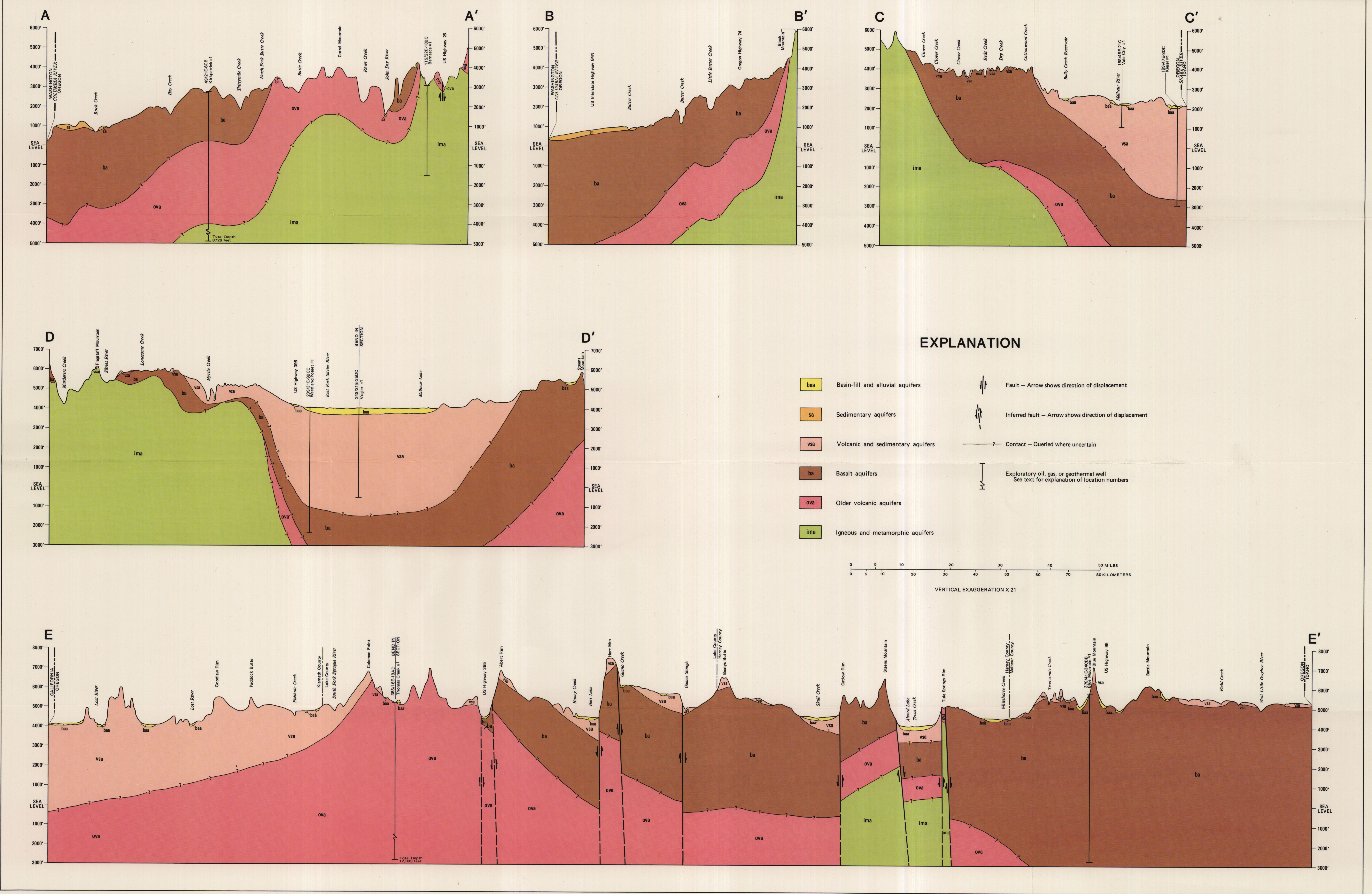
GEOLOGIC CROSS SECTIONS OF AQUIFER UNITS IN EASTERN OREGON (LOCATIONS ON PLATE 1)
