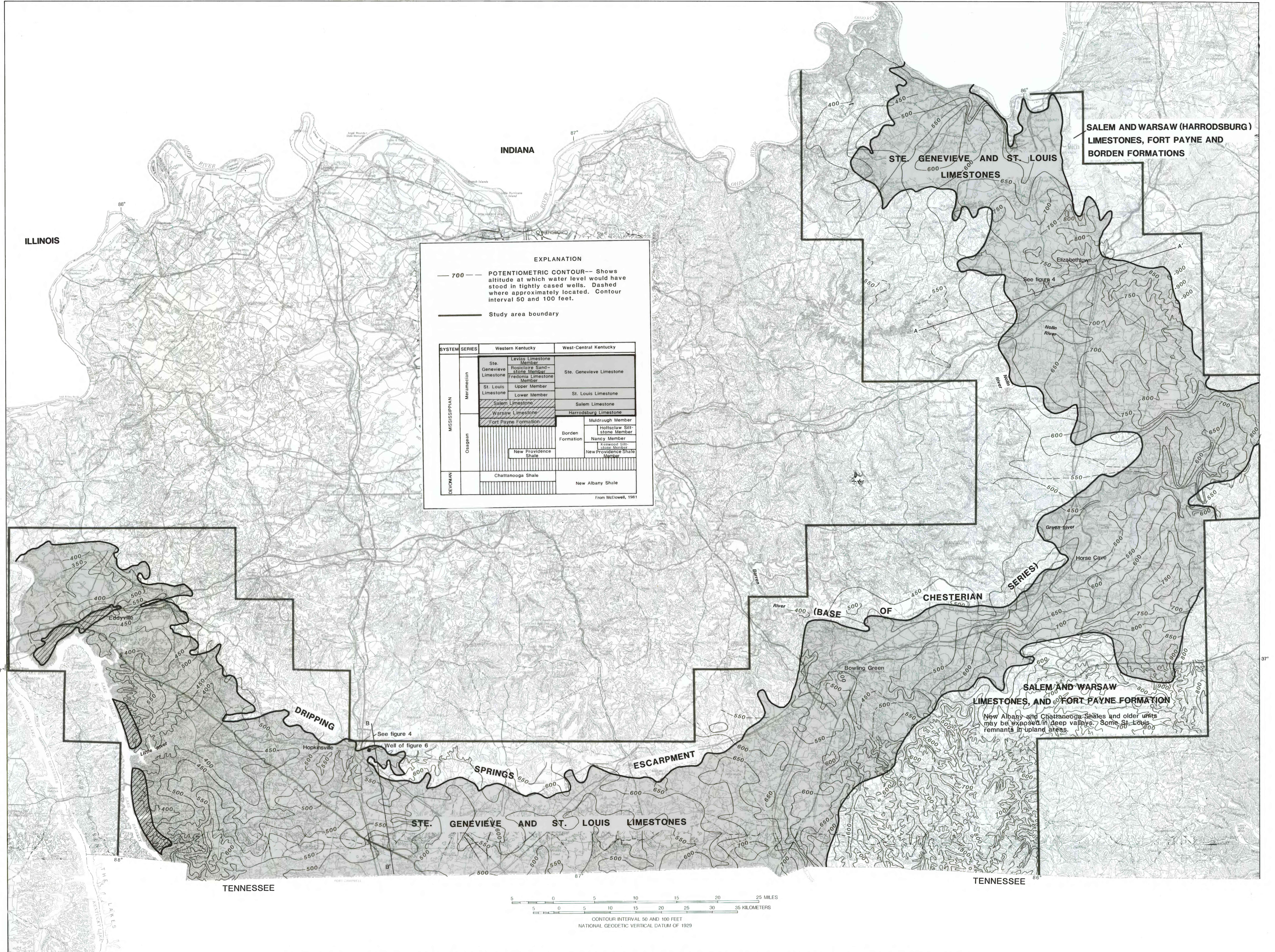
GENERALIZED GEOLOGY AND CONFIGURATION OF THE POTENTIOMETRIC SURFACE IN THE PRINCIPAL AQUIFER, MISSISSIPPIAN PLATEAUS REGION, KENTUCKY.
