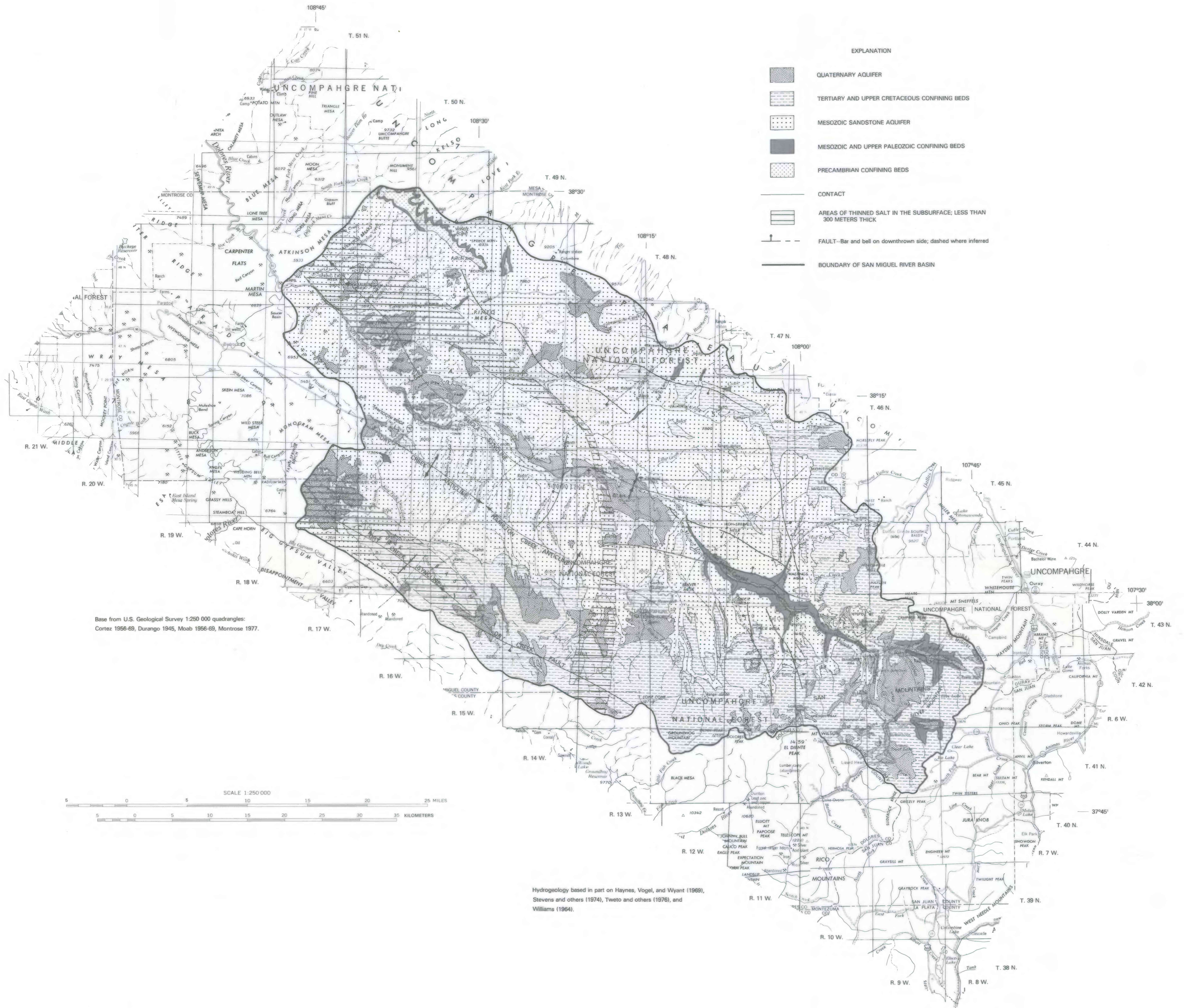
MAP SHOWING GENERALIZED HYDROGEOLOGY OF THE SAN MIGUEL RIVER BASIN, SOUTHWESTERN COLORADO
