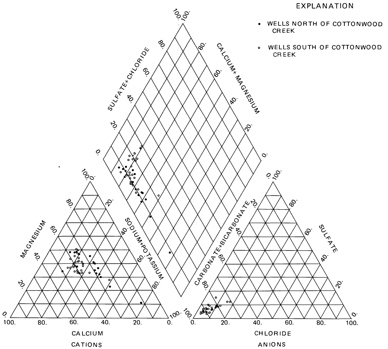
FIGURE 2.-Trilinear diagram showing water quality in the Cottonwood Creek area, October 1982.
