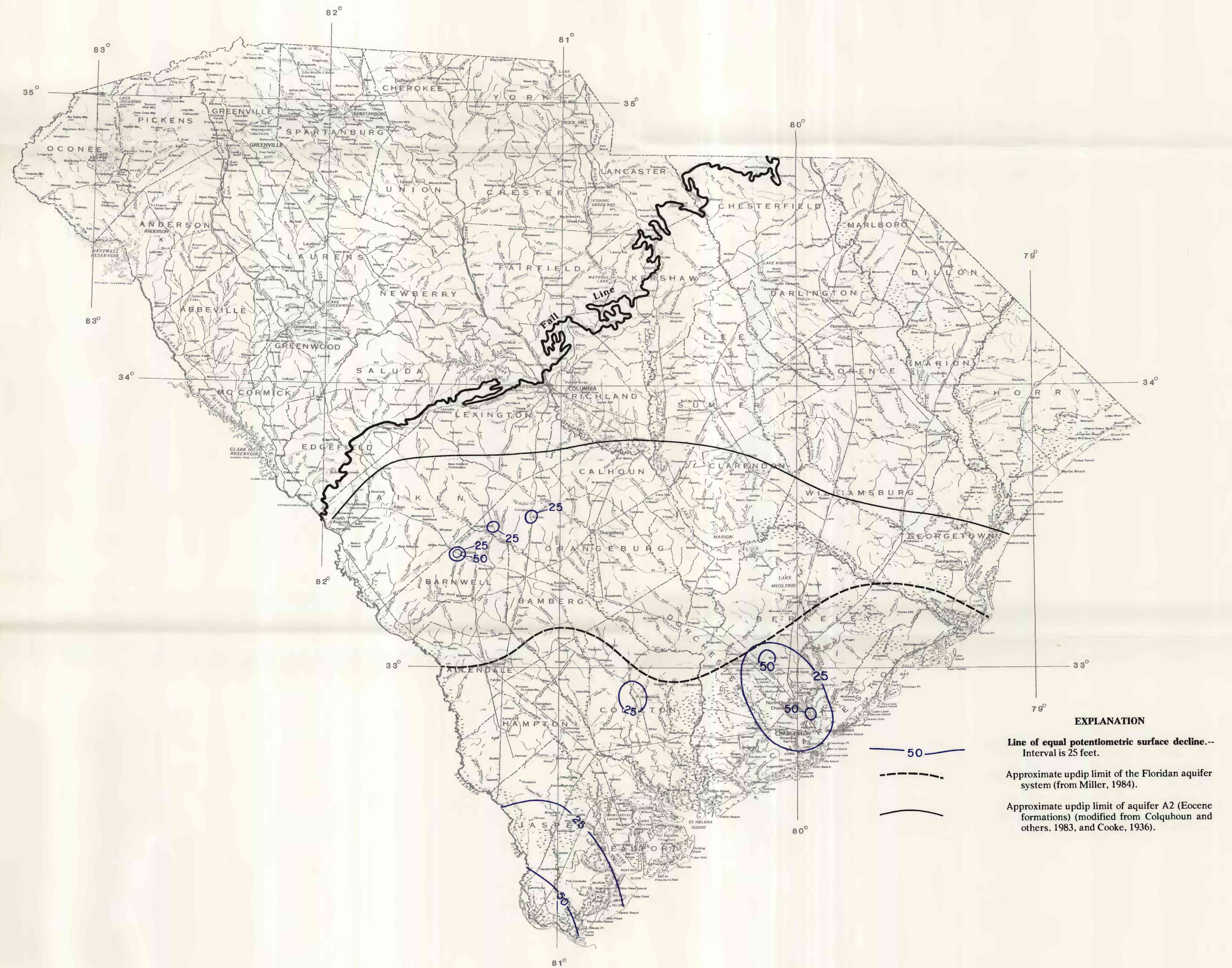
FIGURE 7.--DECLINES IN THE POTENTIOMETRIC SURFACE OF THE FLORIDAN AQUIFER SYSTEM AND AQUIFER A2 (EOCENE FORMATIONS) BETWEEN THE PERIOD PRIOR TO DEVELOPMENT AND NOVEMBER 1982
