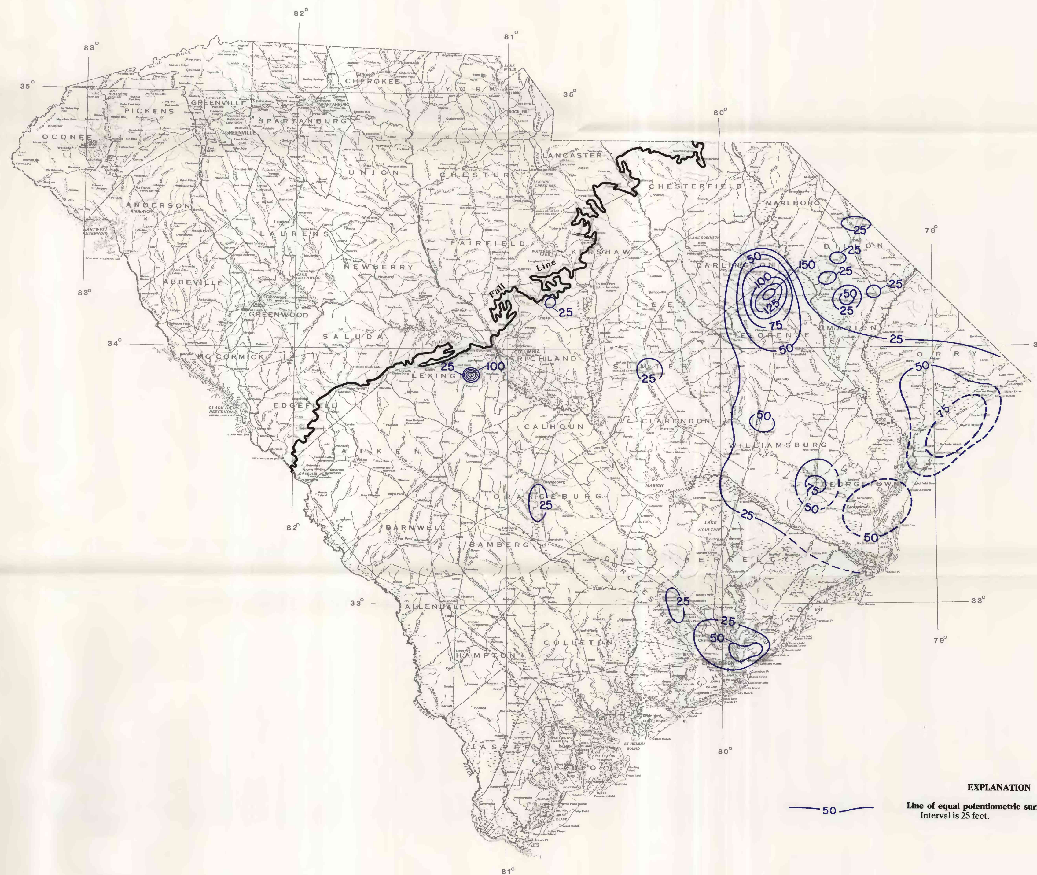
FIGURE 9.--DECLINES IN THE POTENTIOMETRIC SURFACE OF AQUIFER A3a3 (MIDDENDORF FORMATION) BETWEEN THE PERIOD PRIOR TO DEVELOPMENT AND NOVEMBER 1982
