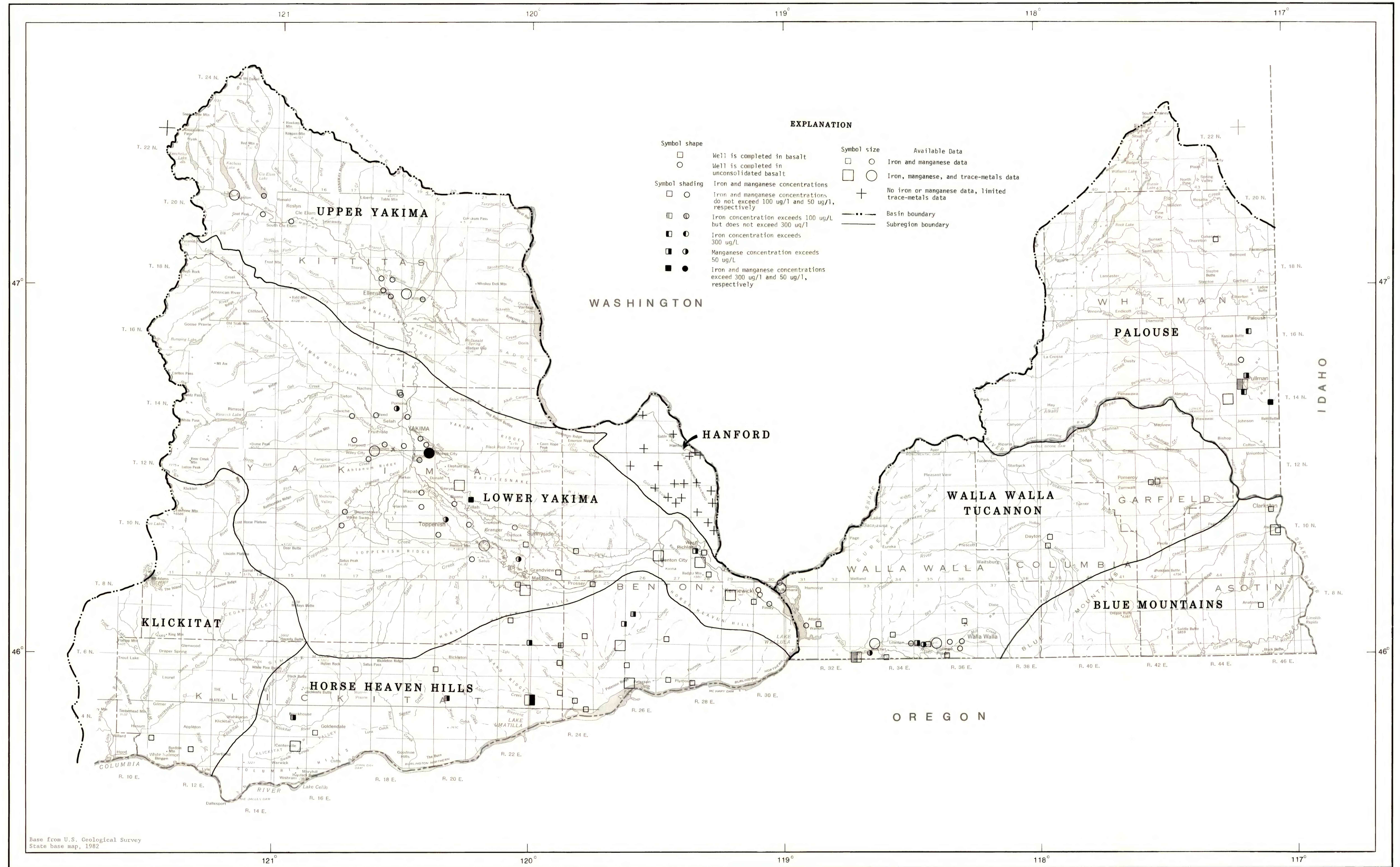
PLATE 3.--Concentrations of iron, manganese, and trace metals in 1982.
