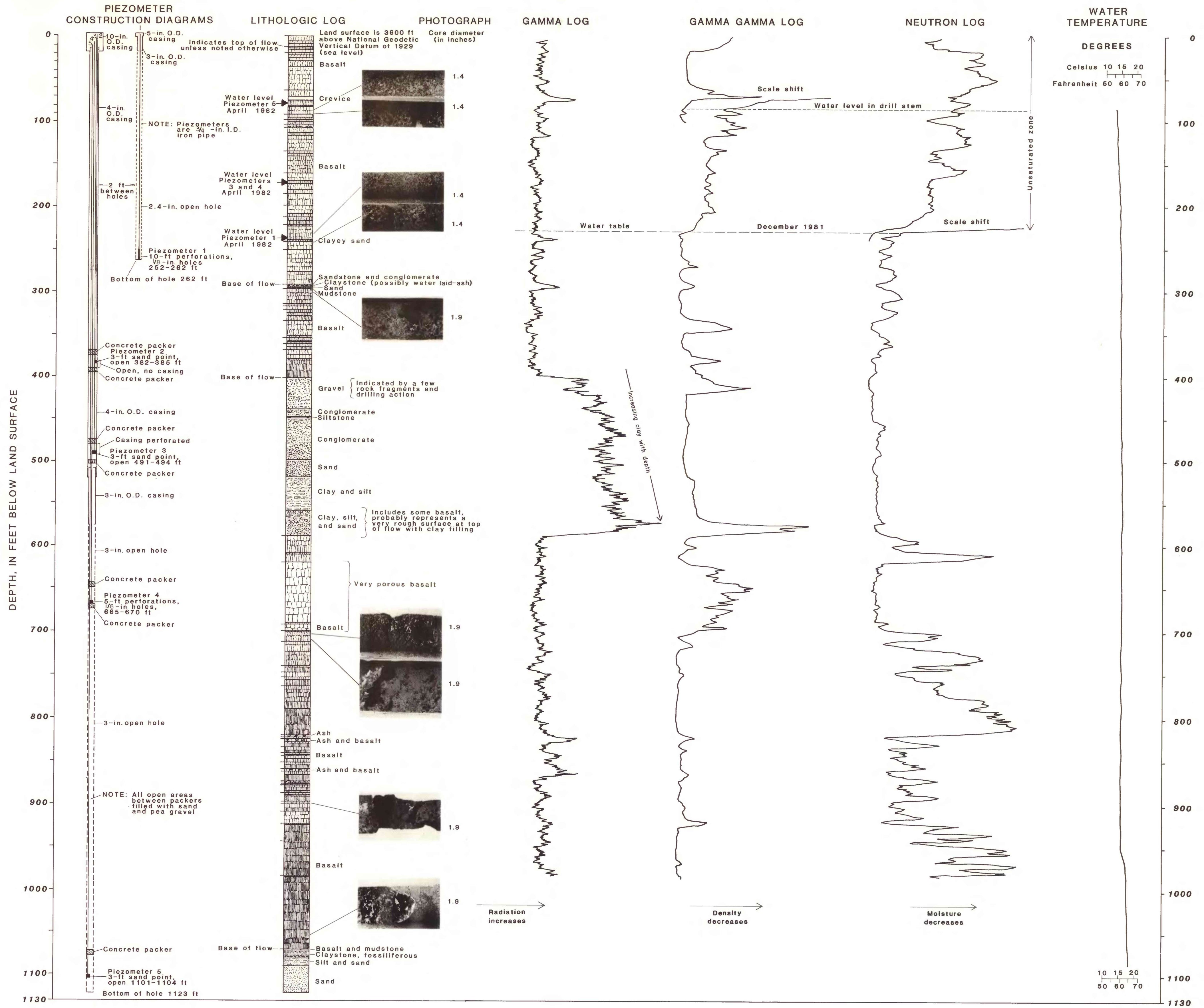
COMPLETION DIAGRAM OF TEST HOLE SHOWING LITHOLOGIC AND GEOPHYSICAL LOGS AND WATER-TEMPERATURE PROFILE
