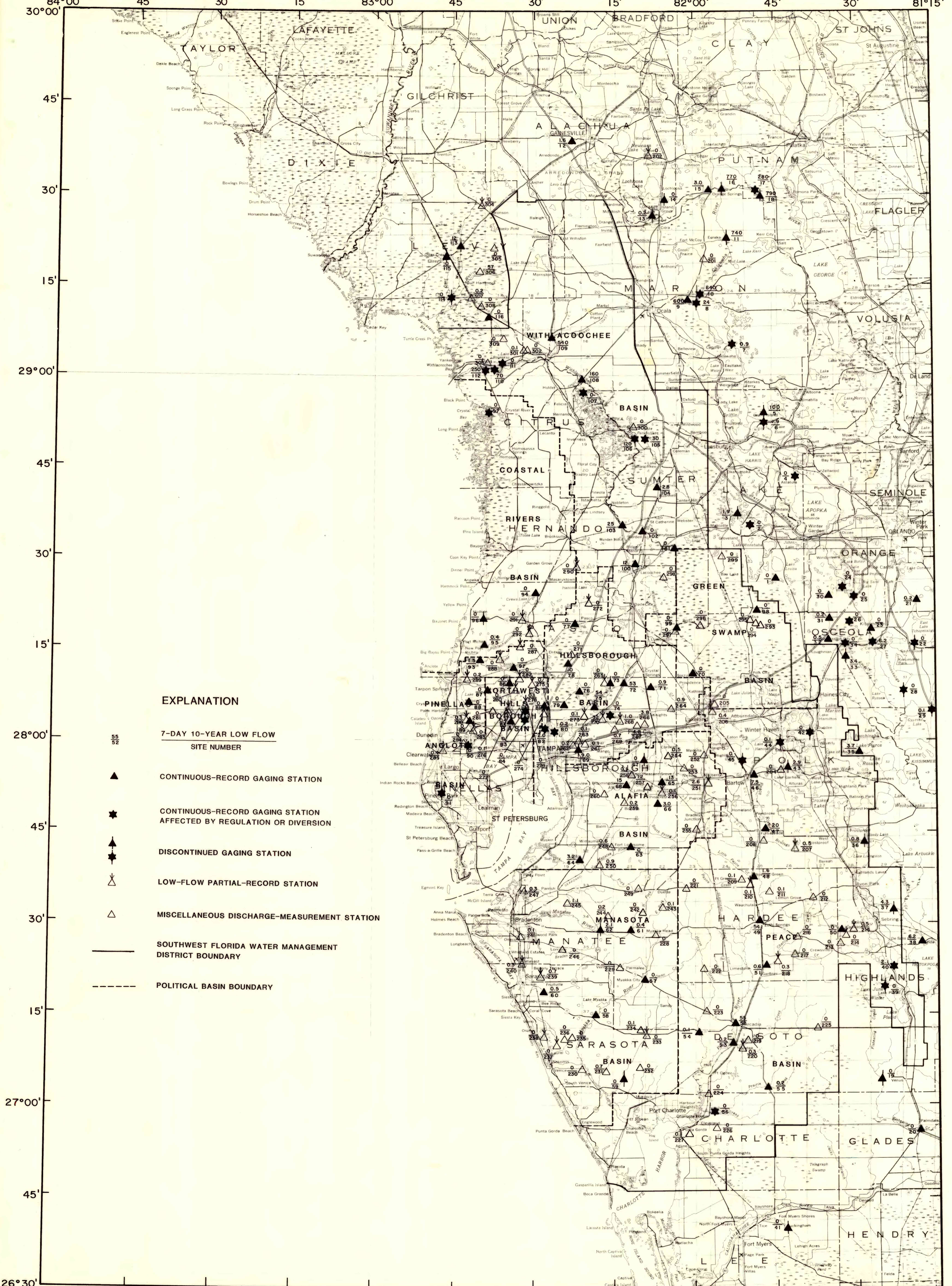
Figure 5.--Seven-day, 10-year low flow at streamflow stations.
