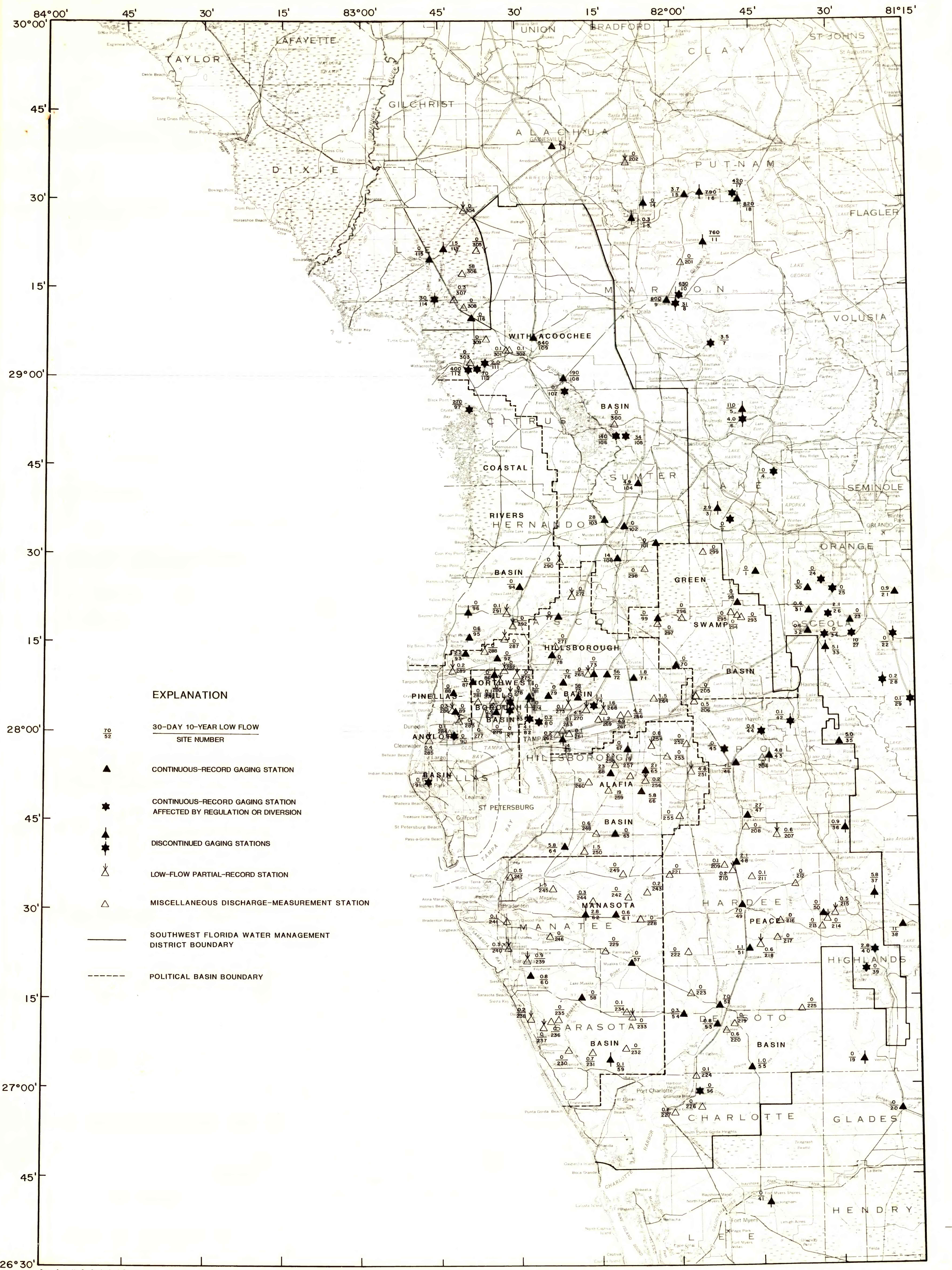
Figure 6.--Thirty-day, 10-year low flow at streamflow stations.
