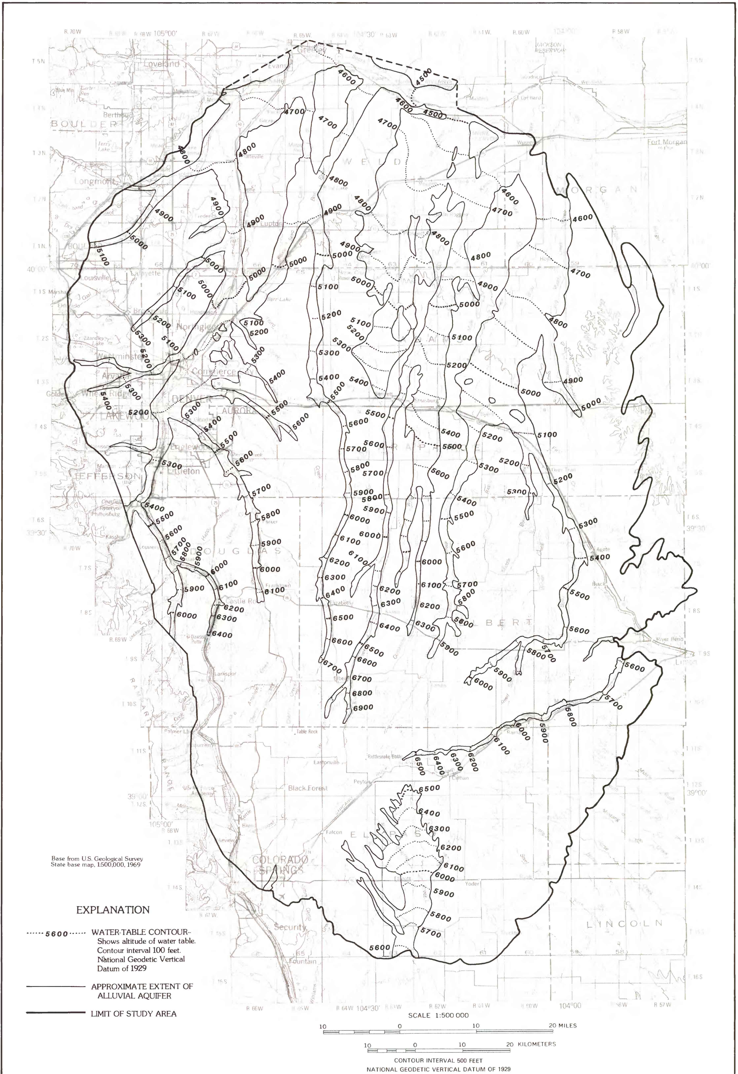
MAP SHOWING APPROXIMATE EXTENT AND WATER-TABLE ALTITUDES OF MAJOR ALLUVIAL AQUIFERS, DENVER COAL REGION, COLORADO
