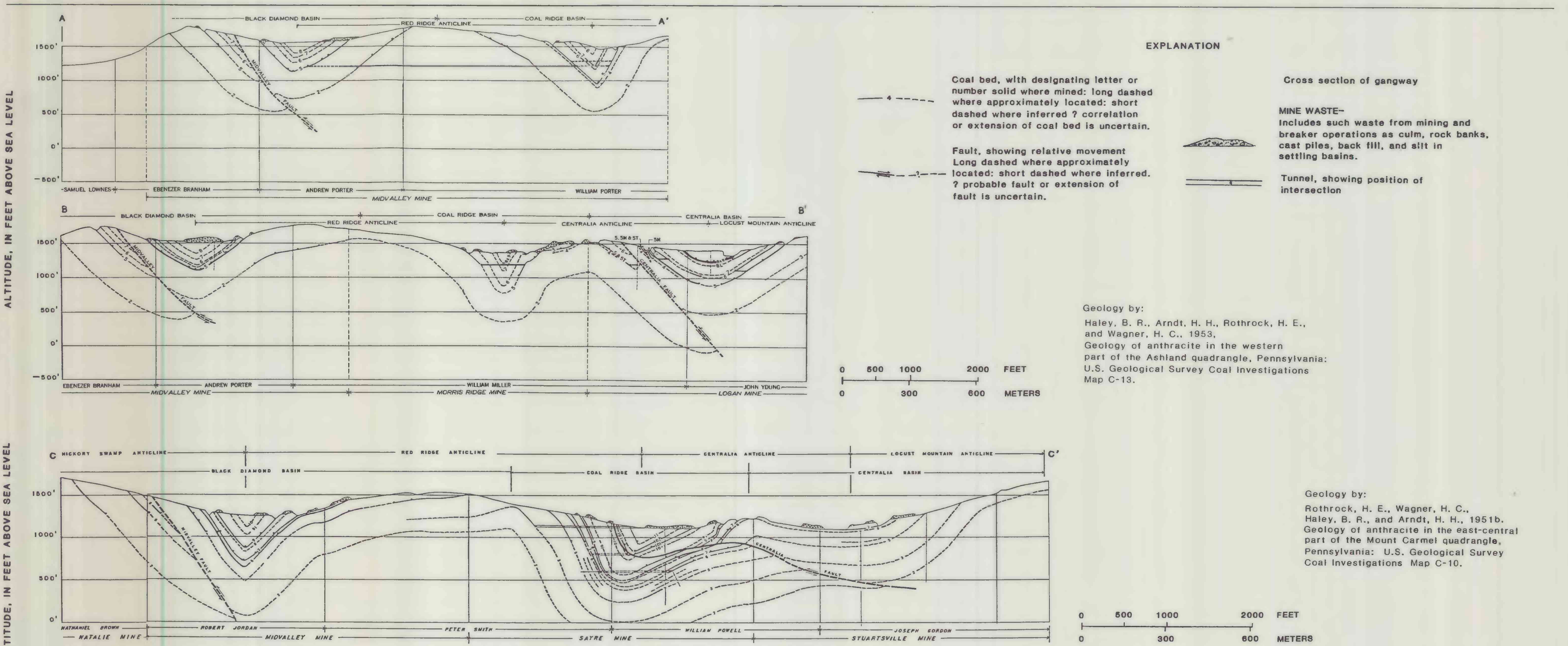
Figure 27.--Structural geologic sections east of Mount Carmel.
