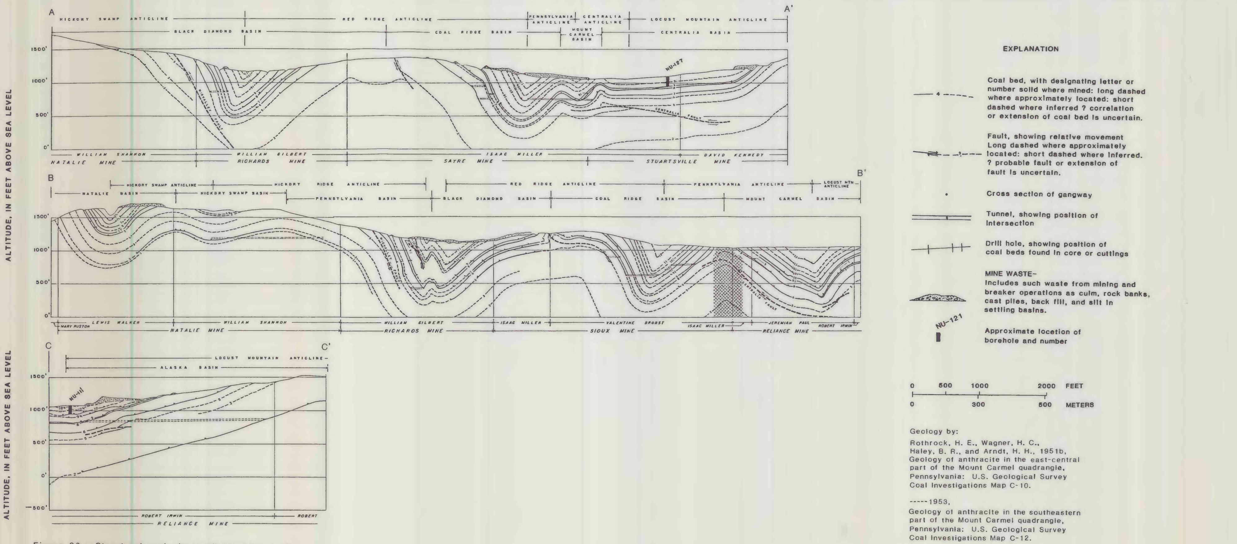
Figure 28.--Structural geologic sections at Mount Carmel.
