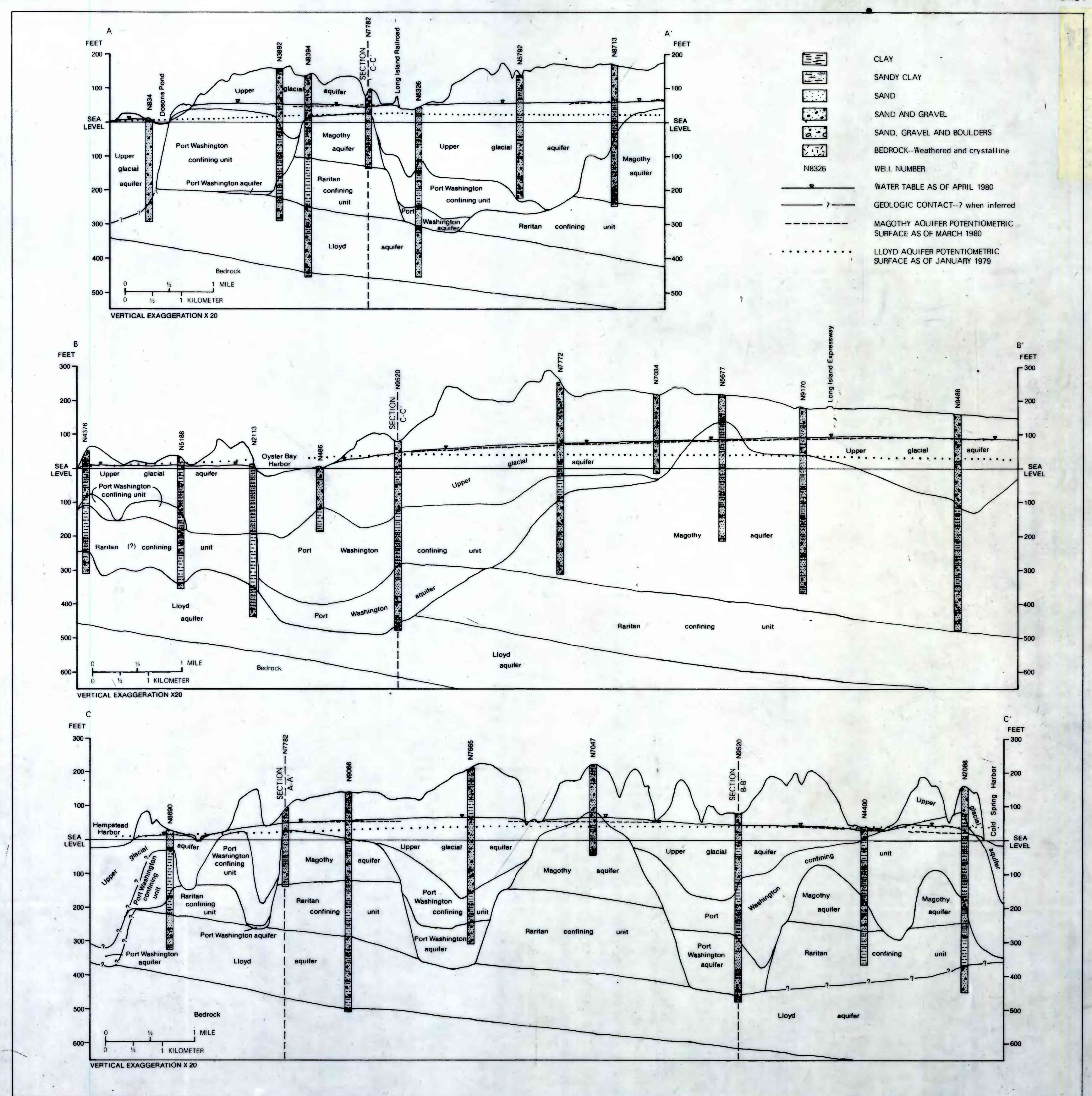
PLATE 1B. HYDROGEOLOGIC SECTIONS A-A', B-B', AND C-C'
