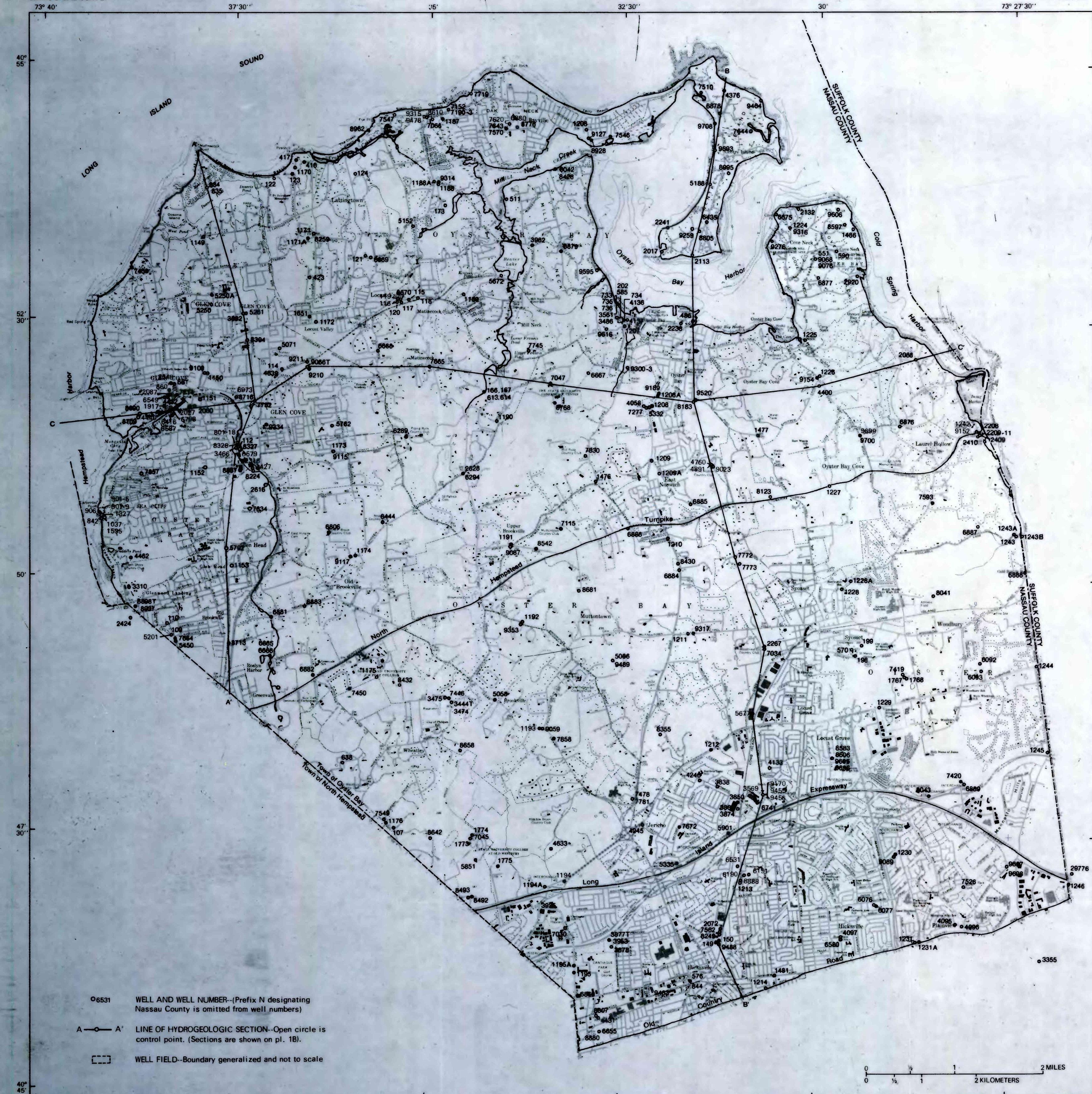
PLATE 1A. LOCATIONS OF SELECTED WELLS AND TEST HOLES AND OF HYDROGEOLOGIC SECTIONS
