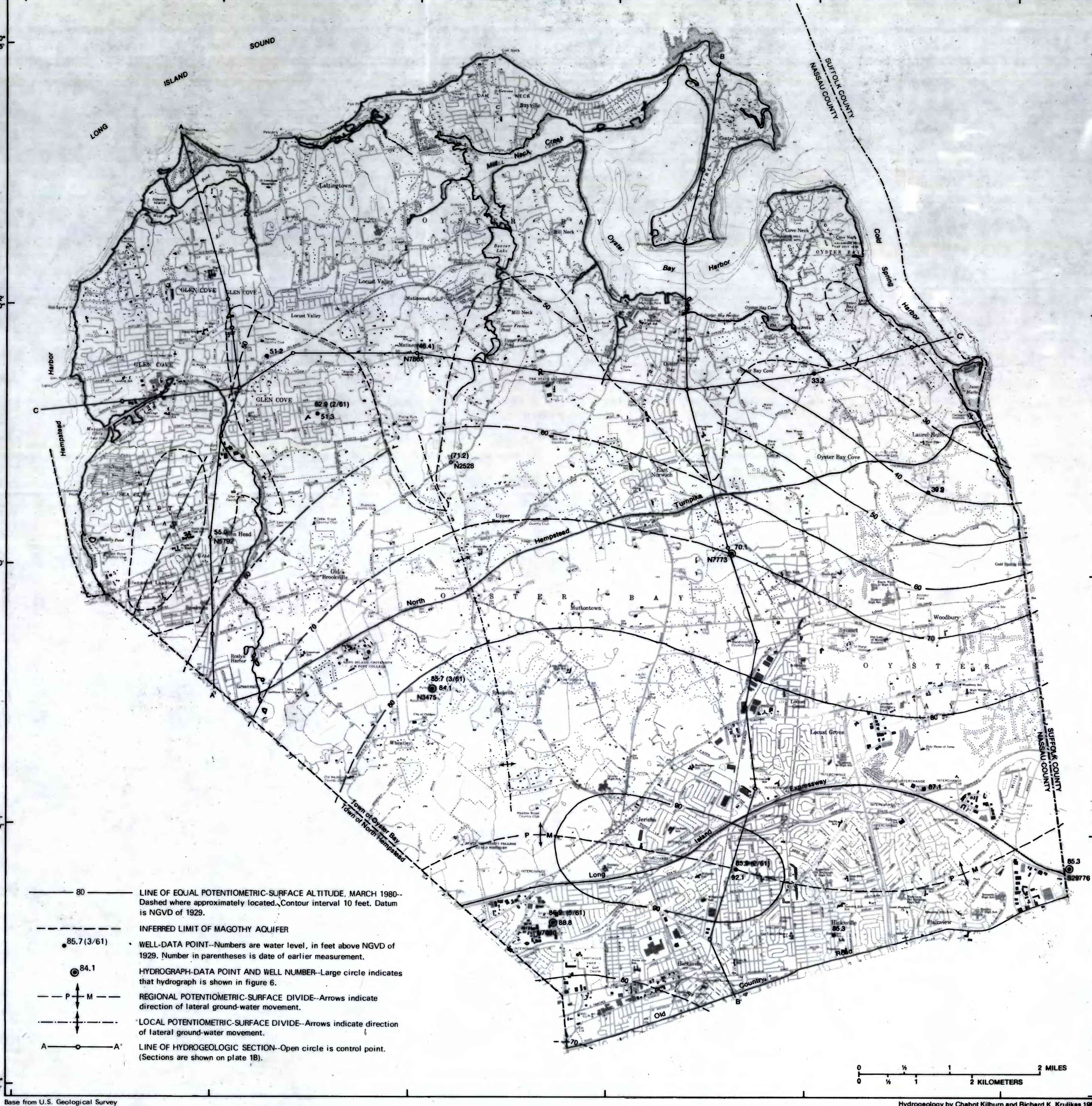
PLATE 5A. POTENTIOMETRIC SURFACE OF THE LOWER PART OF THE MAGOTHY AQUIFER
