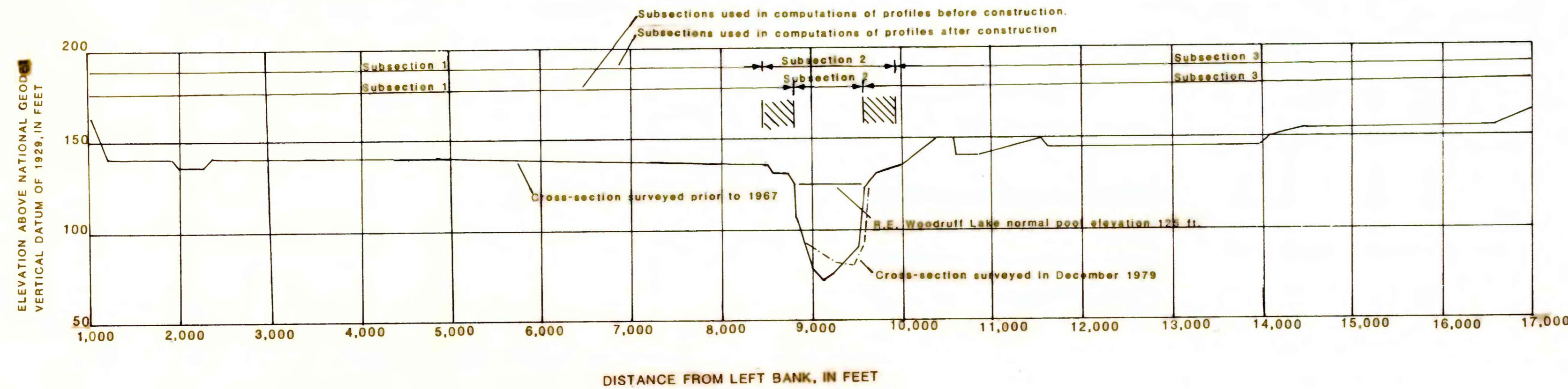
Figure 15.- Elevation of flood plain with subsection rating curves at river mile 264.33.
