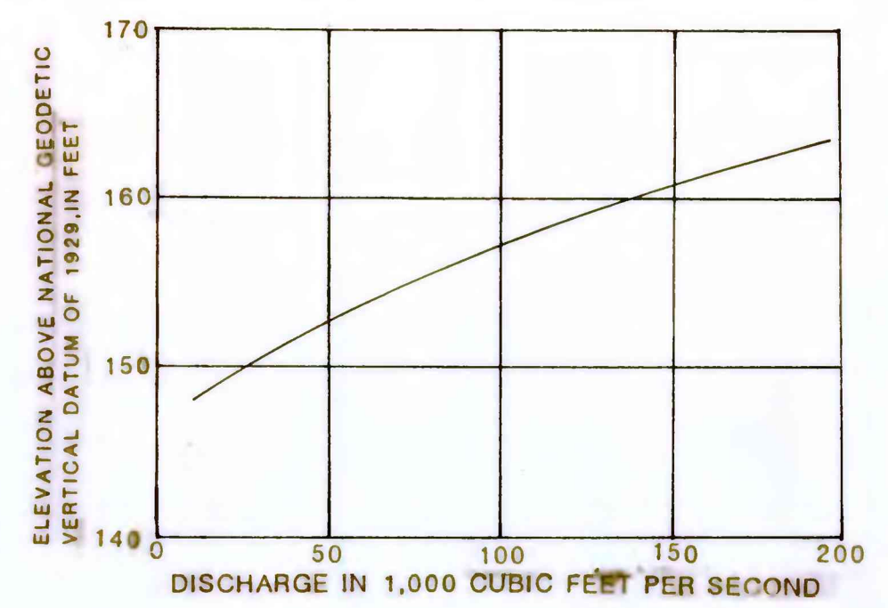
Rating curve for right bank
