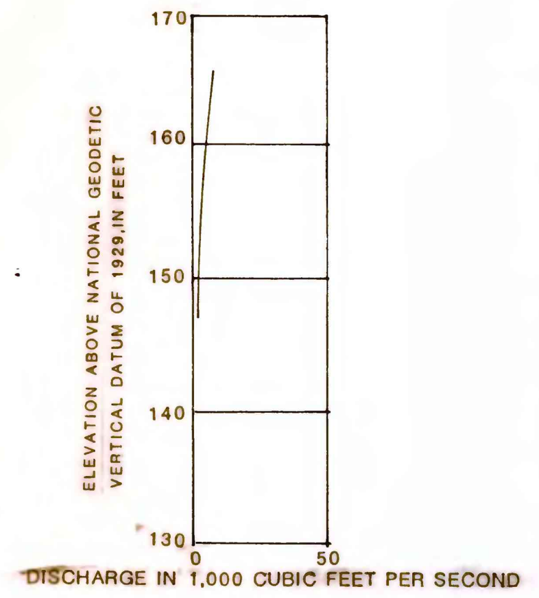
Rating curve for left bank
