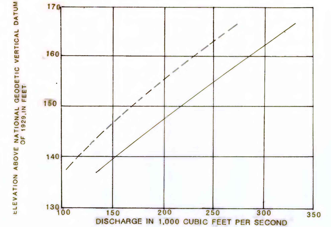
Rating curve for main channel
