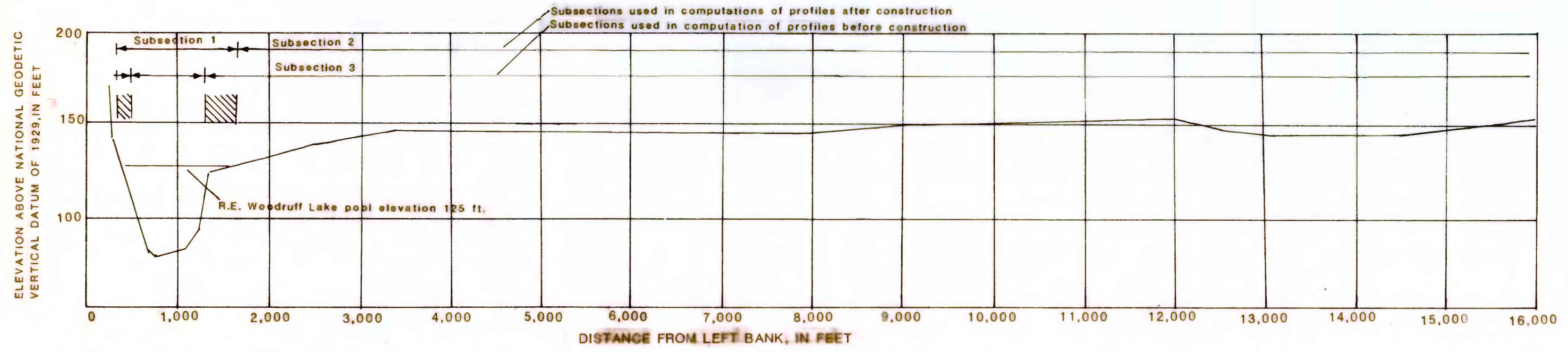
Figure 16.- Elevation of flood plain with subsection rating curves at river mile 280.9
