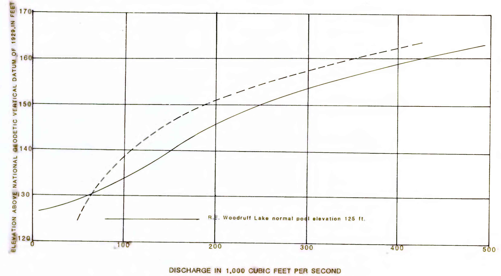
Rating curves for valley cross section.
