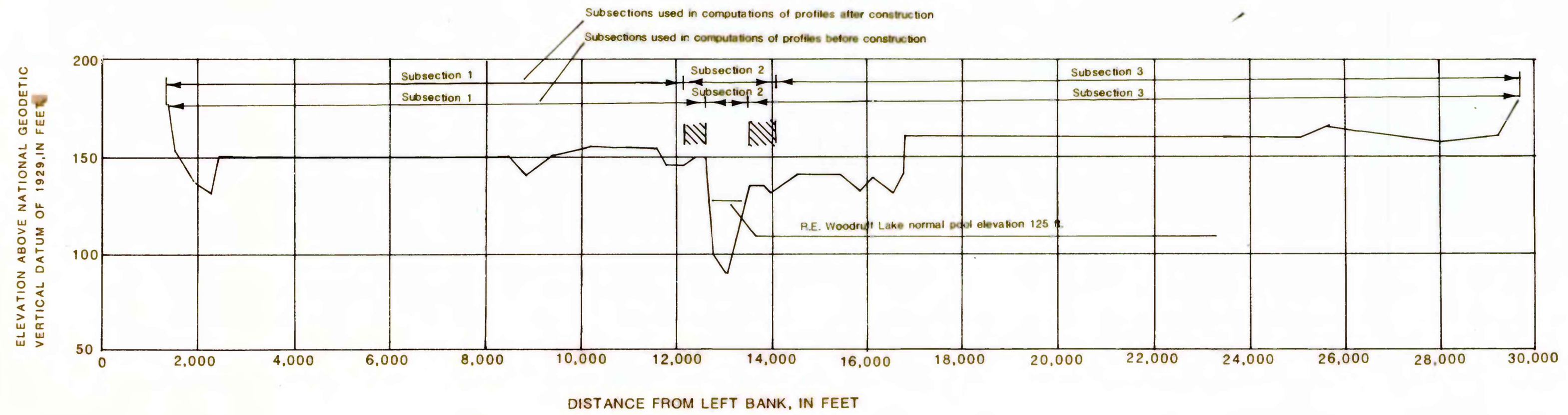
Figure 17.- Elevation of flood plain with subsection rating curves at river mile 308.0
