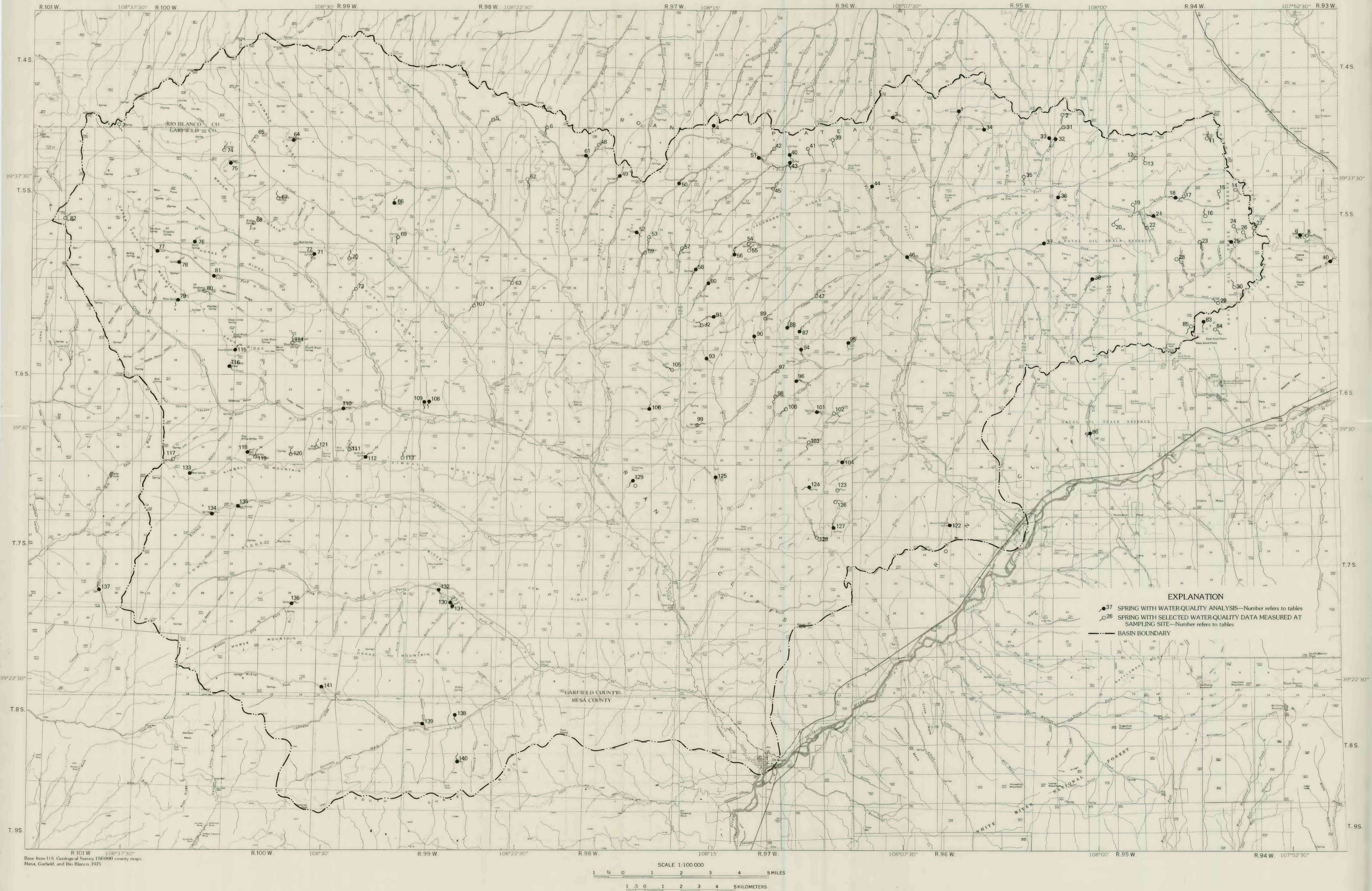
MAP SHOWING LOCATION OF SPRINGS INVENTORIED AND SAMPLED IN ROAN AND PARACHUTE CREEK BASINS, NORTHWESTERN COLORADO, 1981-83
