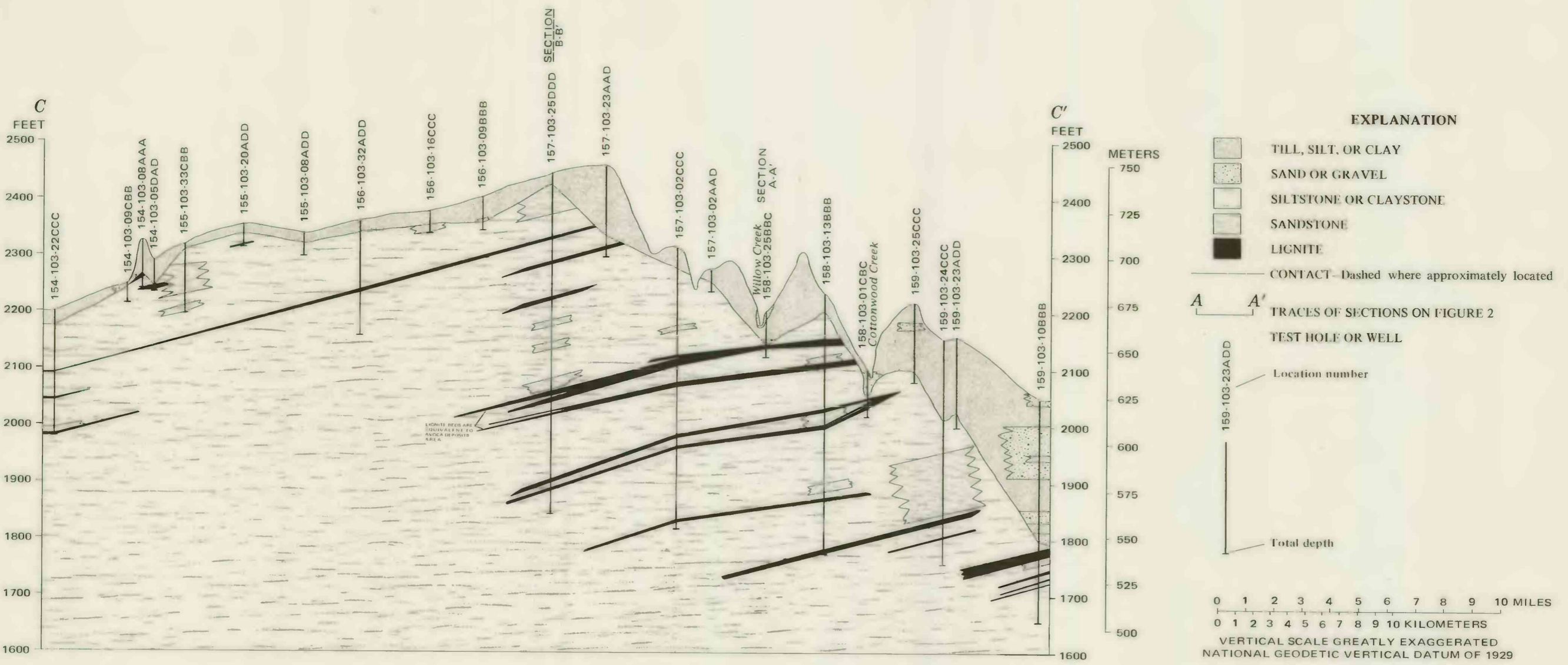
LITHOLOGIC SECTIONS, SAND CREEK-HANKS LIGNITE AREA, WESTERN WILLIAMS COUNTY, NORTH DAKOTA
