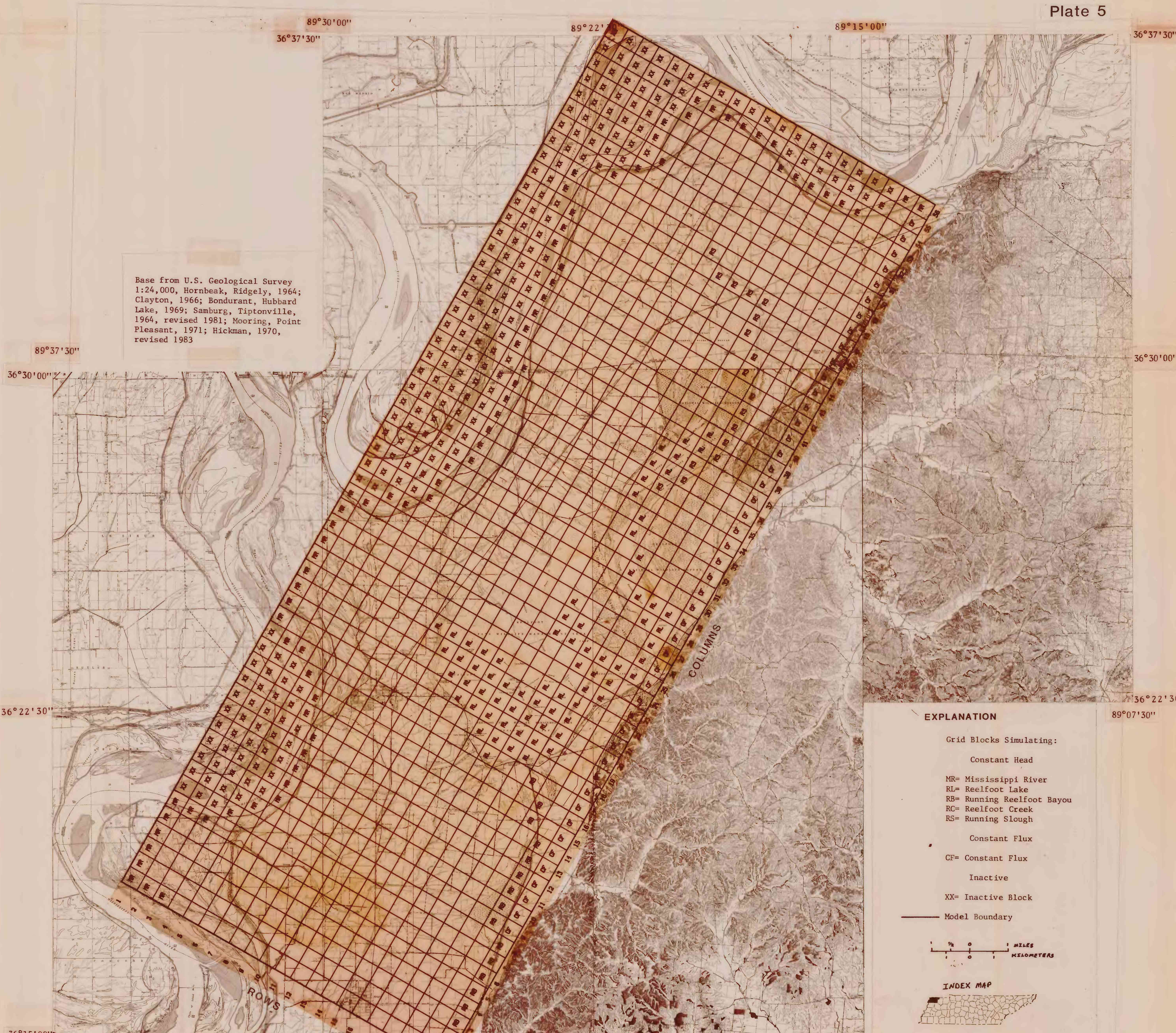
Plate 5.-- Finite-difference grid and model boundaries for the Reelfoot Lake area for the August-September simulation period.
