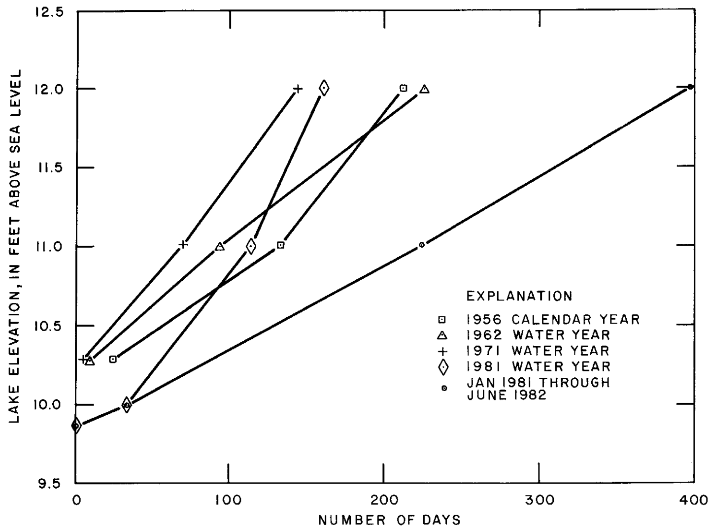
Figure 7.--Number of days water-surface elevation in Lake Okeechobee was at or below indicated elevations in 1956, 1962, 1971, 1981, and January 1981 through June 1982.
