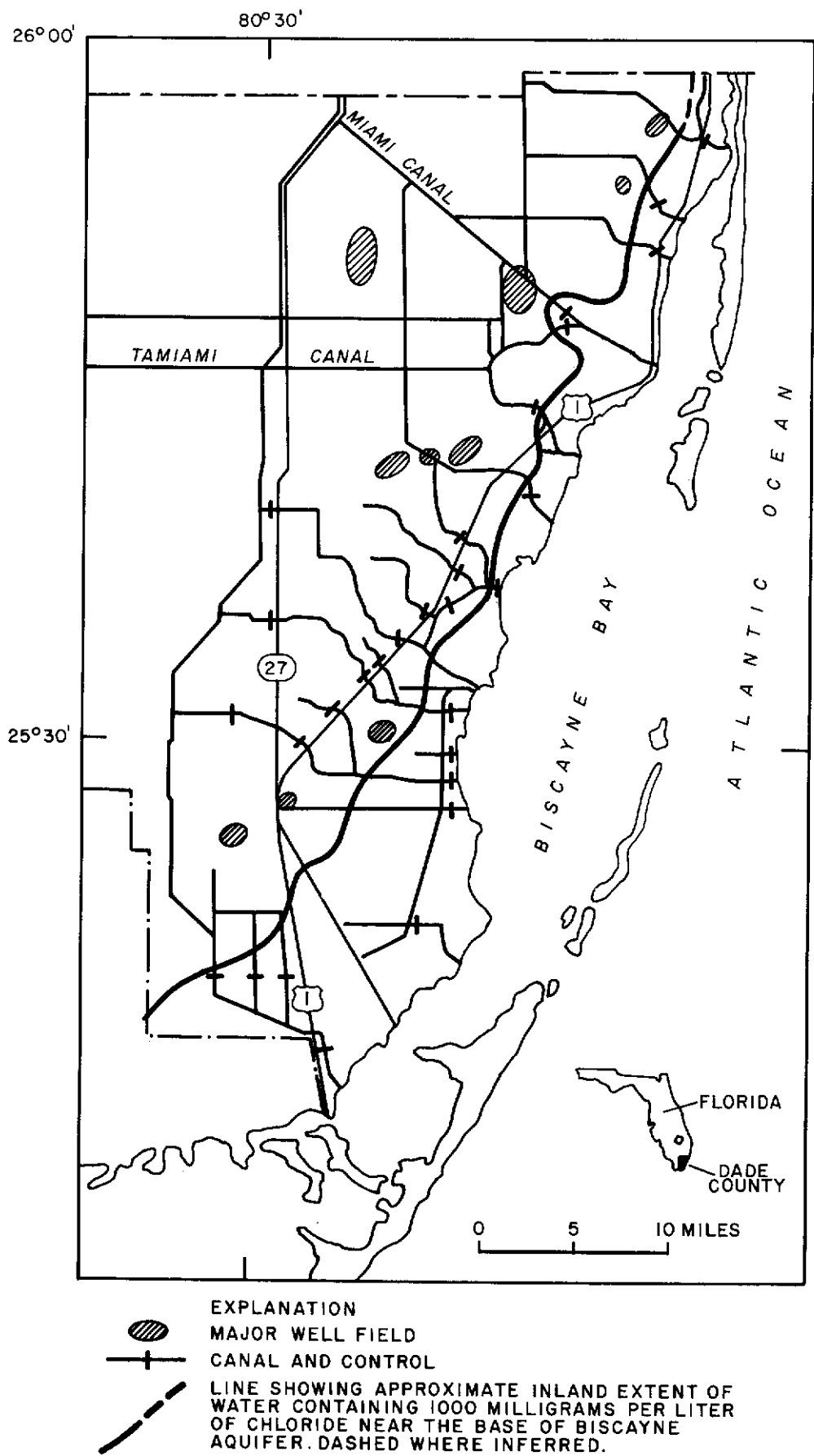
Figure 9.—Saltfront location in Dade County, Florida, March and May 1981.
