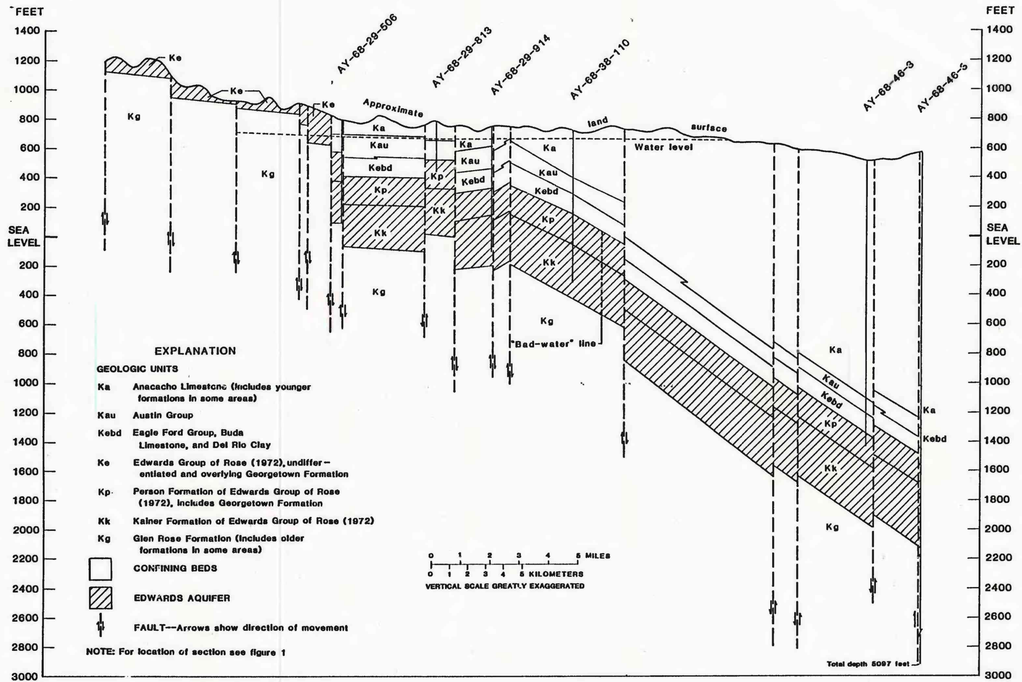
Figure 8.--Hydrogeologic section, F-F'.
