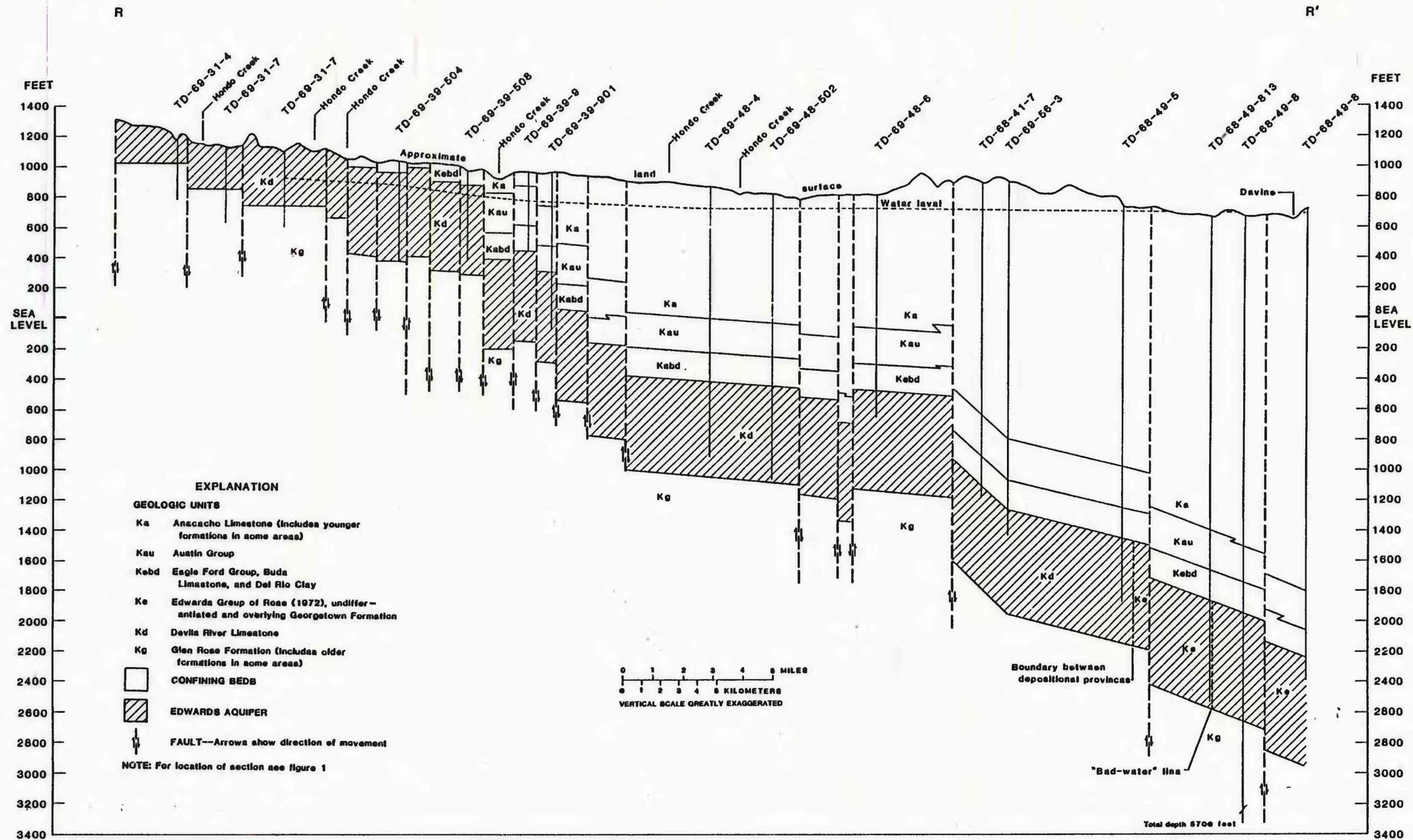
Figure 20.--Hydrogeologic section, R-R'.
