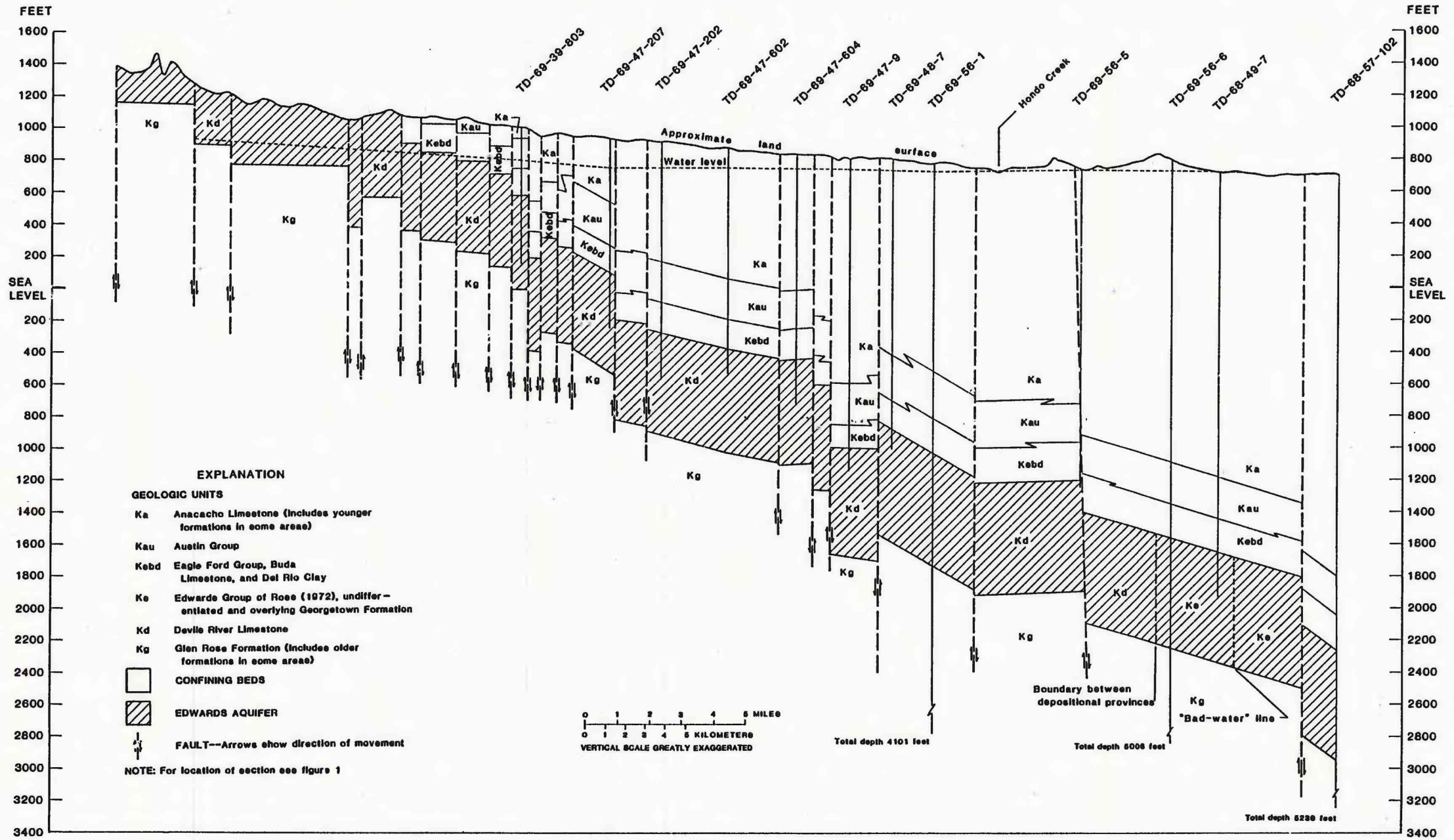
Figure 21.--Hydrogeologic section, S-S'.
