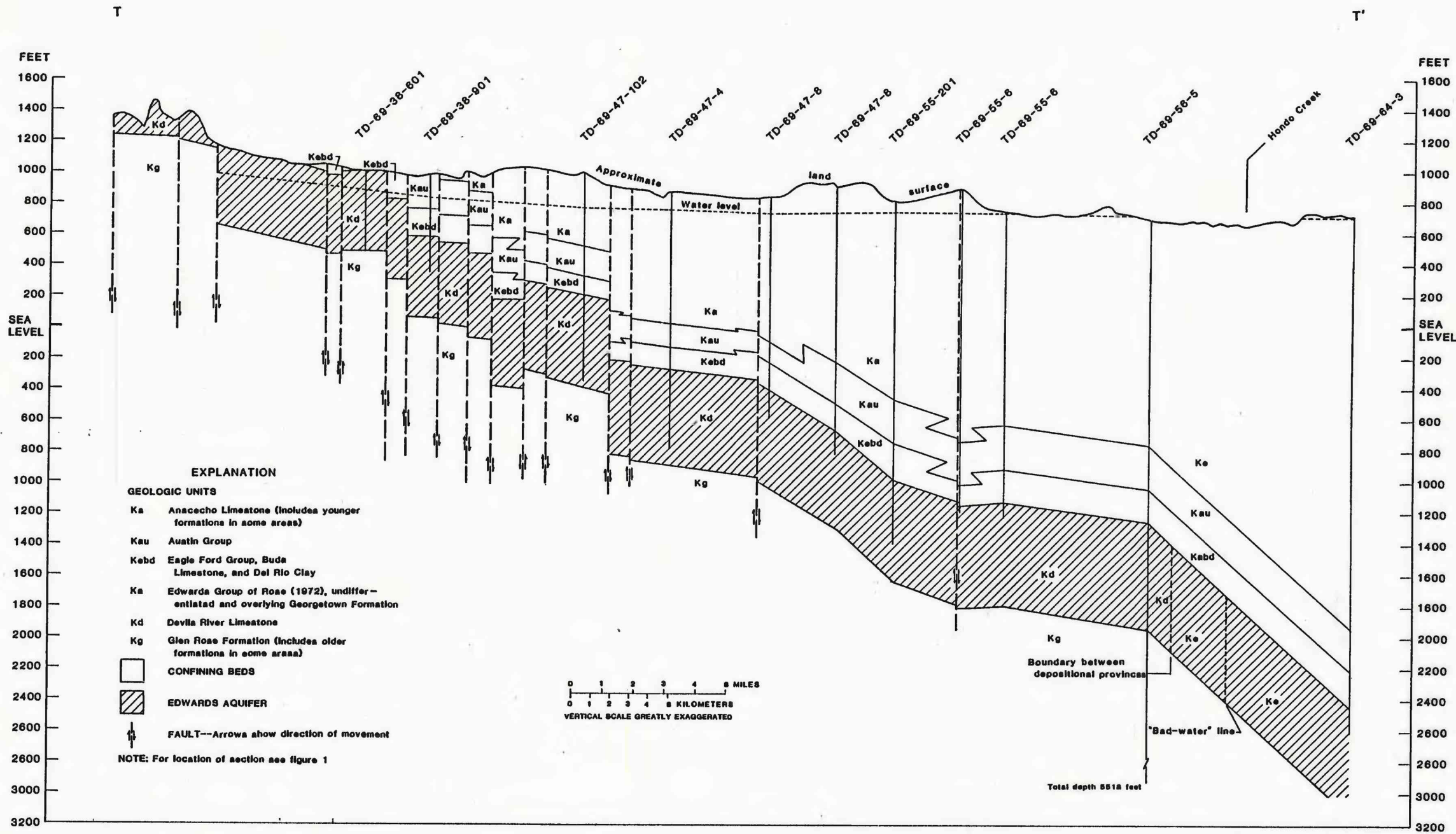
Figure 22.--Hydrogeologic section, T-T'.
