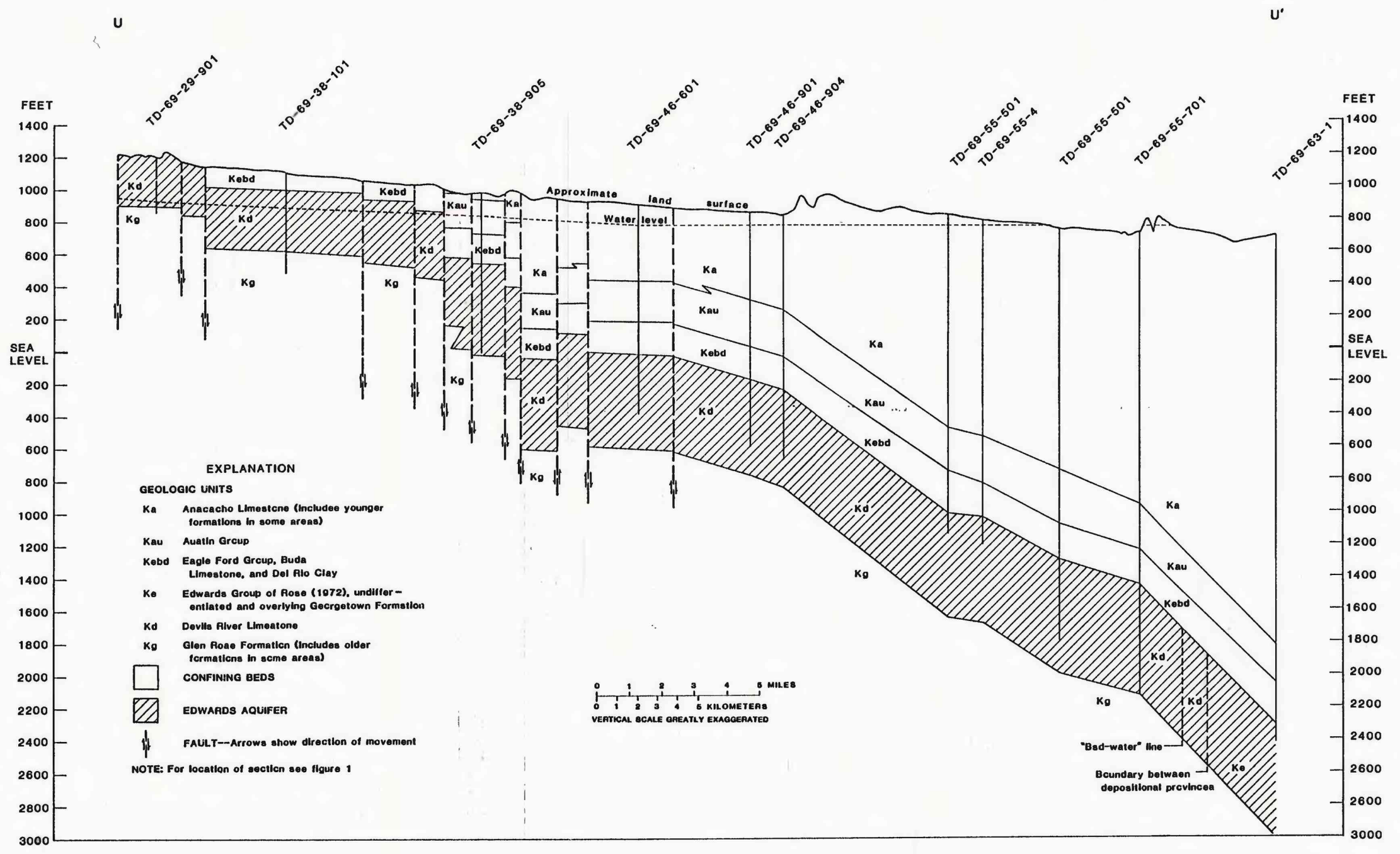
Figure 23.--Hydrogeologic section, U-U'.
