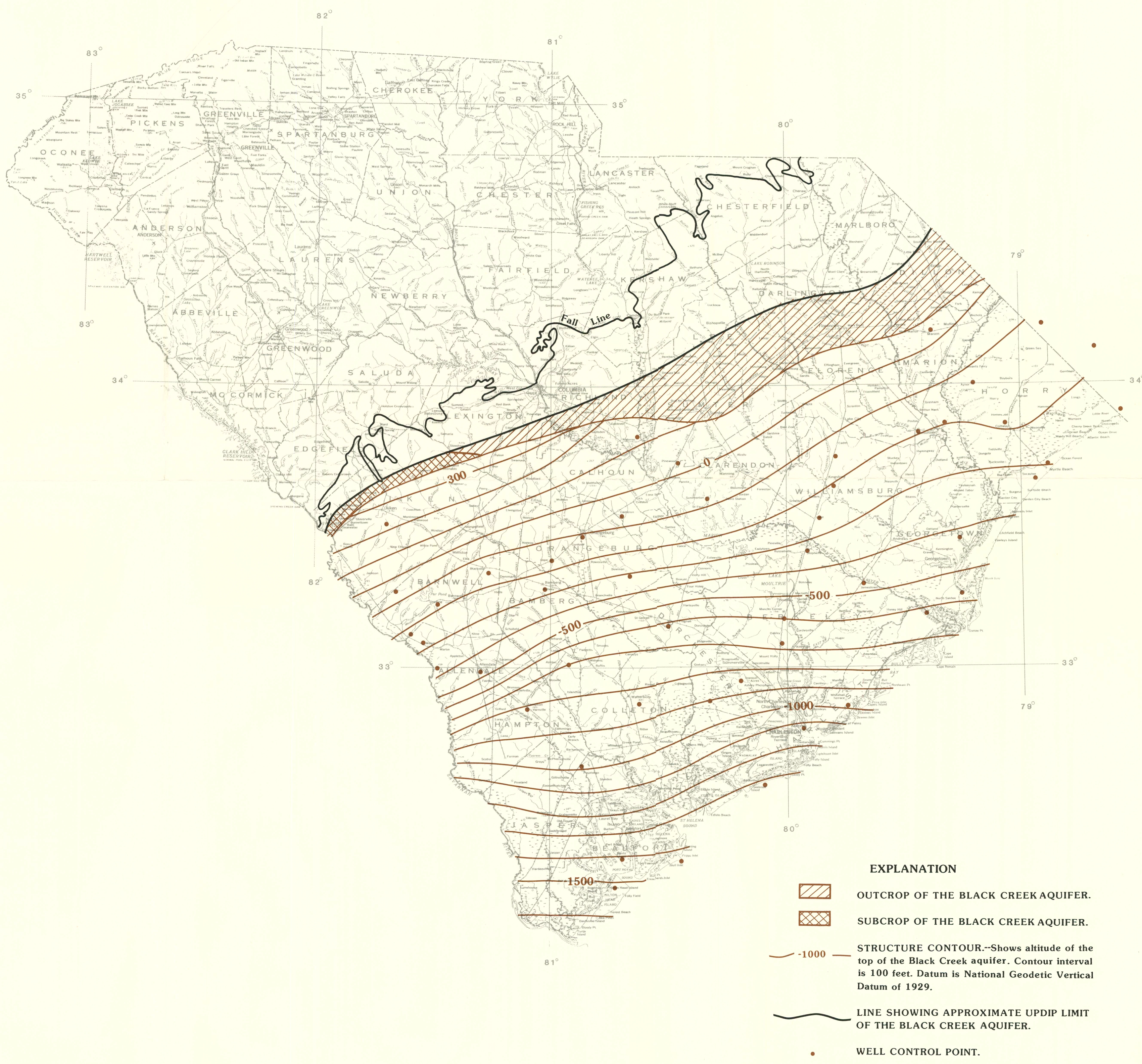
FIGURE 3.--CONFIGURATION OF THE TOP OF THE BLACK CREEK AQUIFER.
