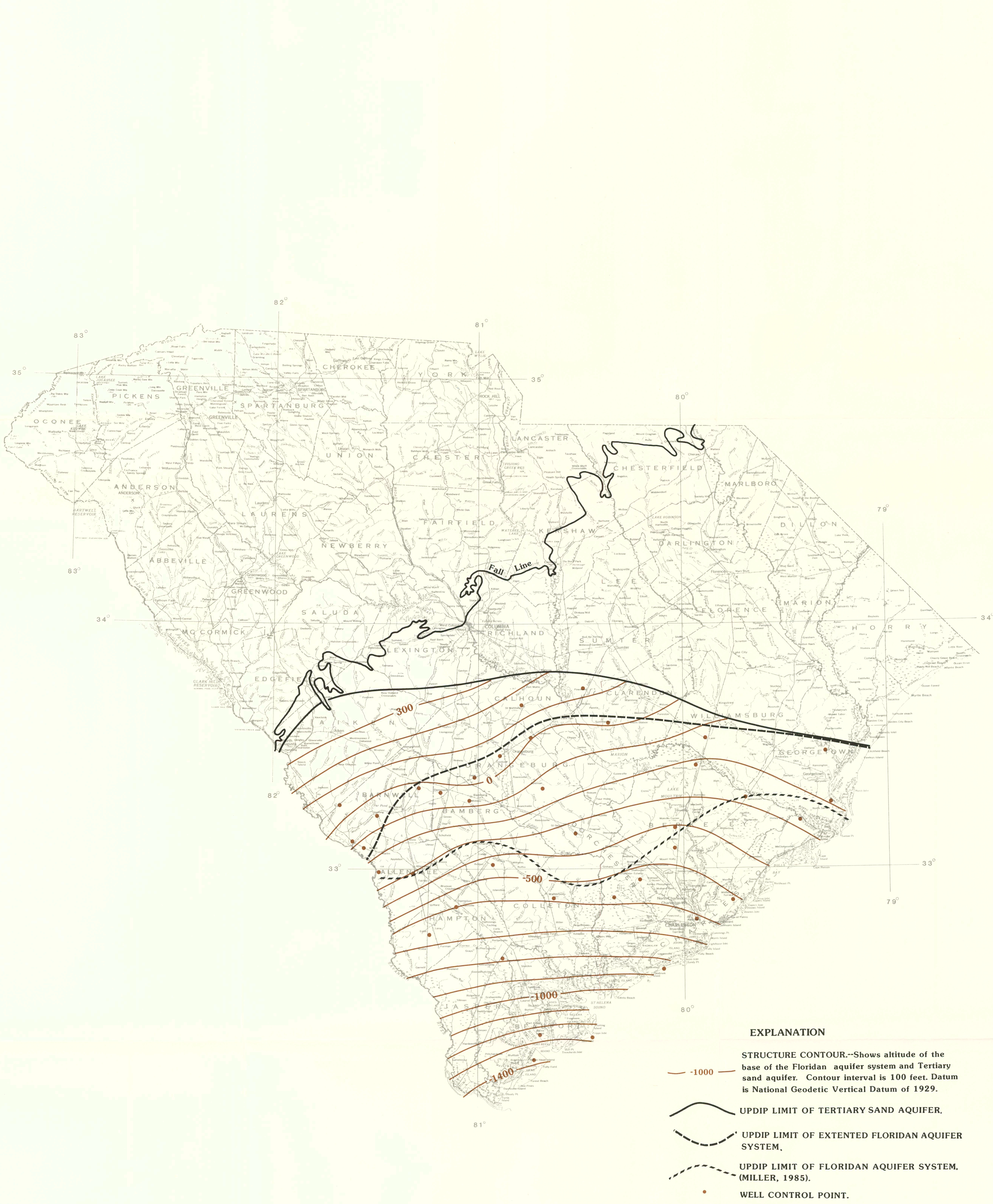
FIGURE 2.--CONFIGURATION OF THE BASE OF THE FLORIDAN AQUIFER SYSTEM AND TERTIARY SAND AQUIFER.
