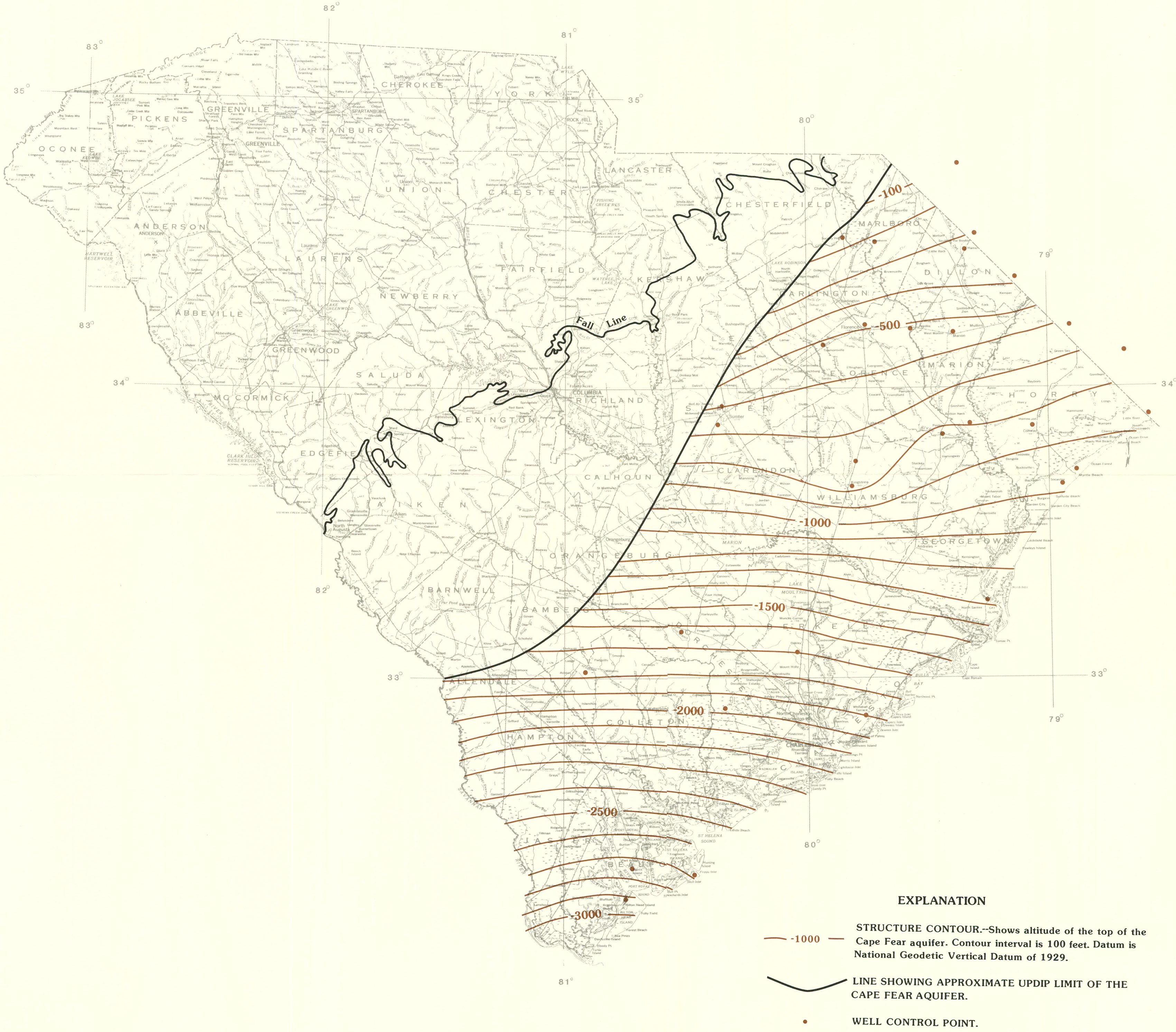
FIGURE 5.--CONFIGURATION OF THE TOP OF THE CAPE FEAR AQUIFER.
