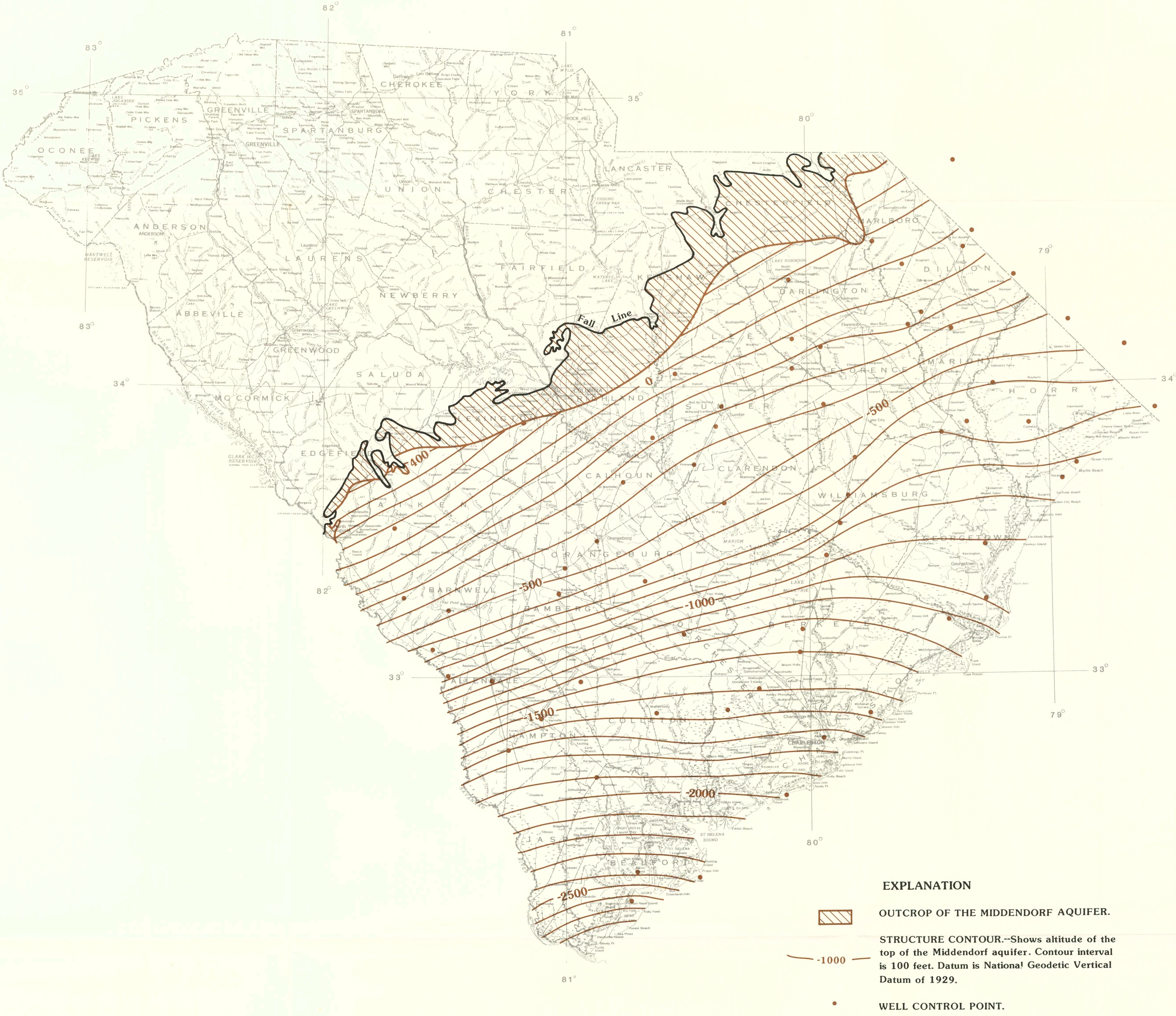
FIGURE 4.--CONFIGURATION OF THE TOP OF THE MIDDENDORF AQUIFER.
