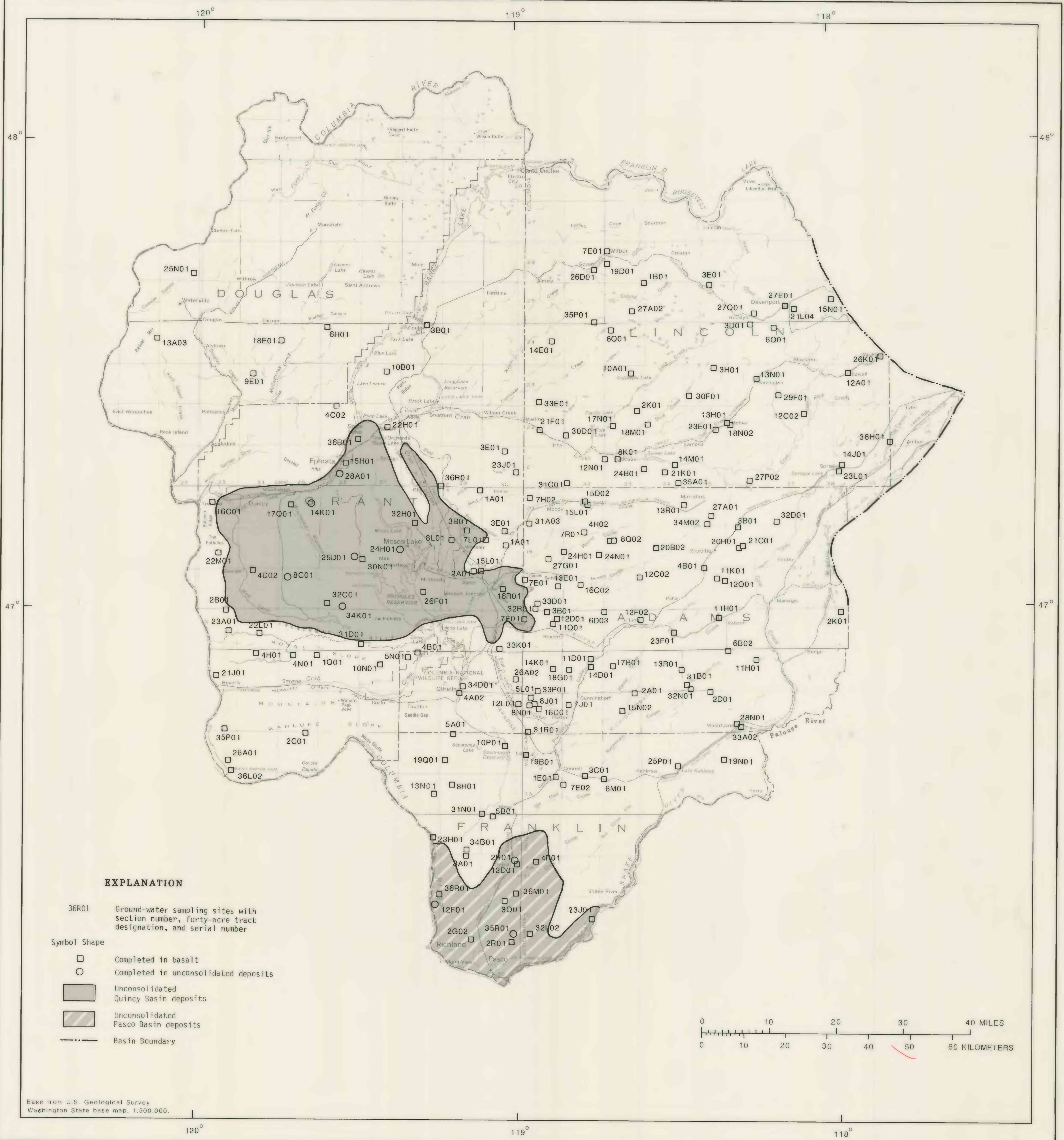
PLATE 1.--Locations of sites with 1983 ground-water quality data.
