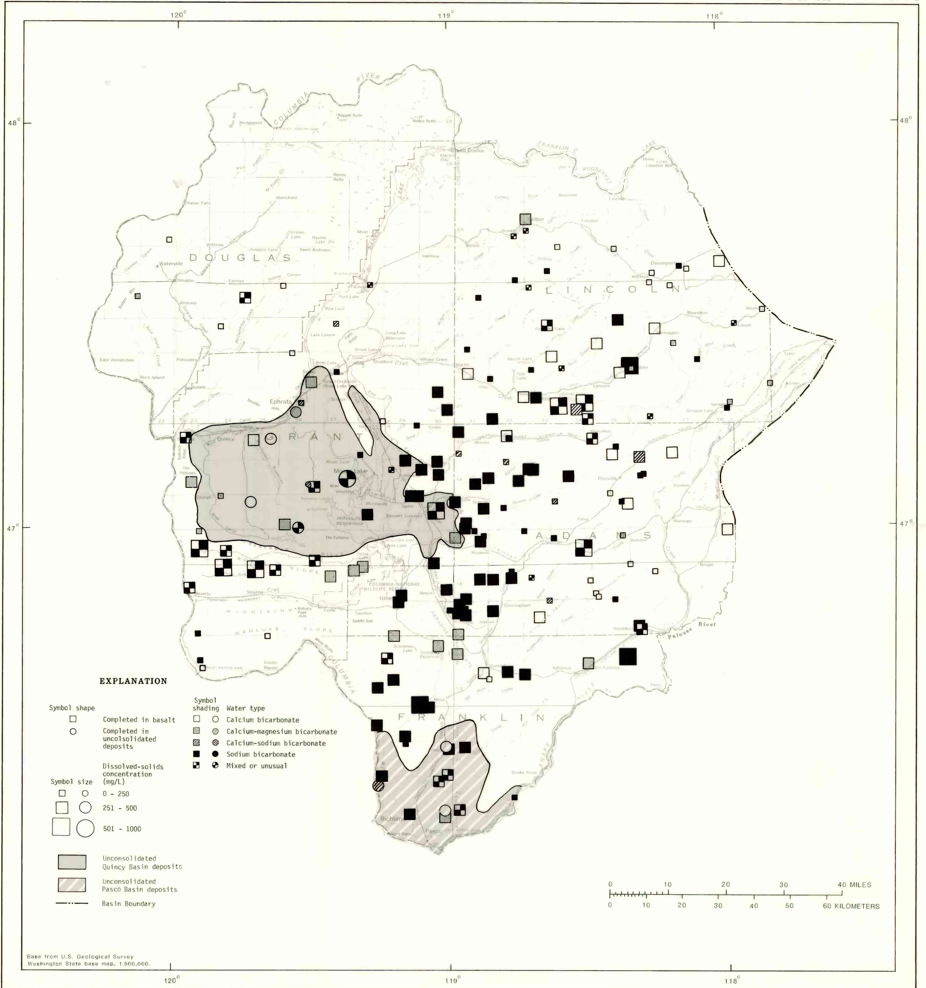
PLATE 2.--Water types and concentrations of dissolved solids.
