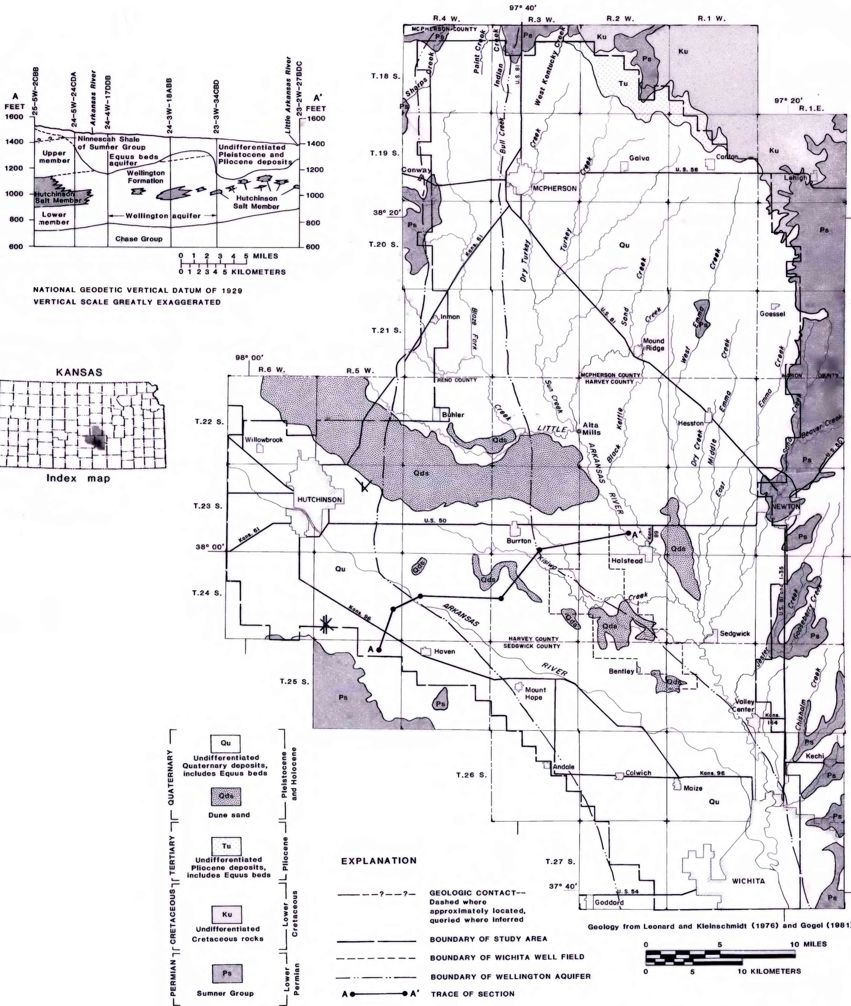
MAP SHOWING SURFICIAL GEOLOGY IN THE EQUUS BEDS AREA, SOUTH-CENTRAL KANSAS By Joseph M. Spinazola, J. B. Gillespie, and R. J. Hart 1985
